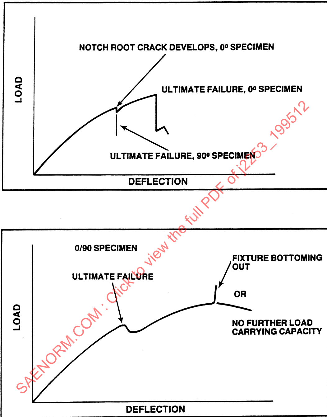
FIGURE 3—TYPICAL SHEAR LOAD-DEFLECTION CURVES
