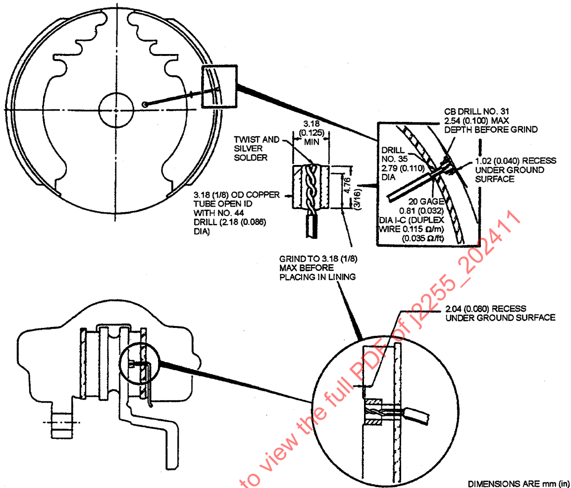
Figure 3 - Typical plug type thermocouple installation
