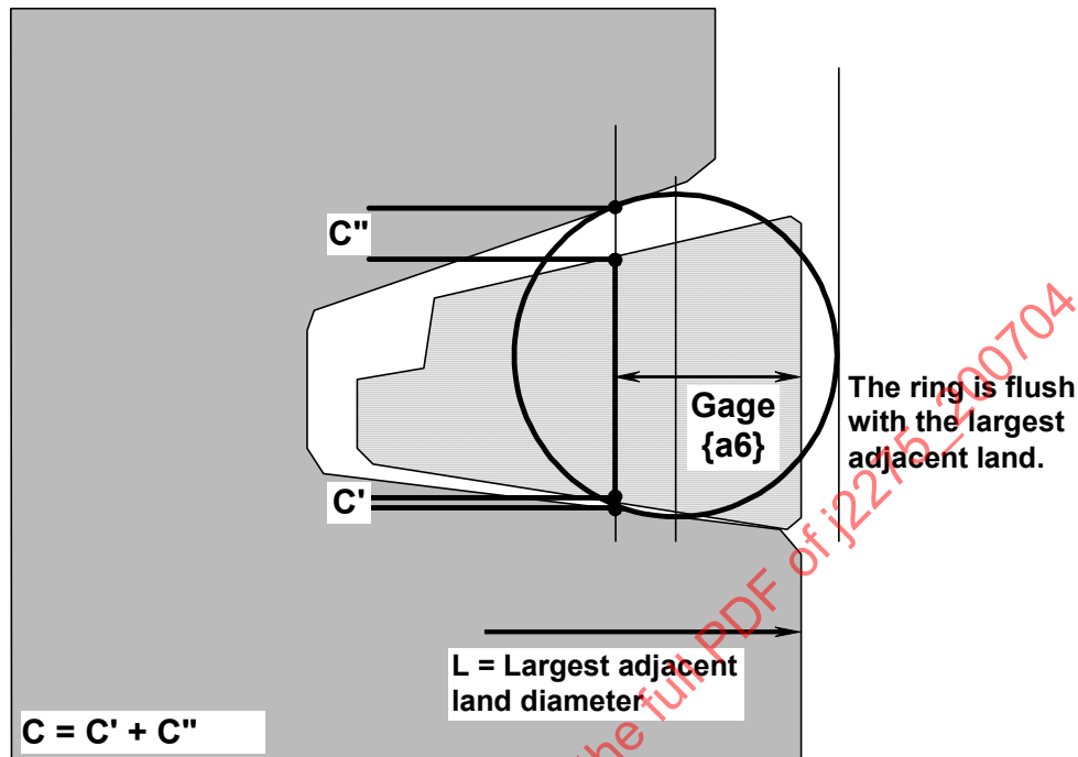
FIGURE 21 - KEYSTONE RING GROOVE CLEARANCE (EXAMPLE CALCULATION)
