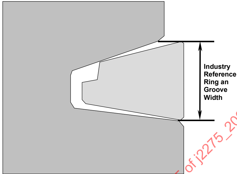
FIGURE 18 - INDUSTRY REFERENCE RING AND GROOVE WIDTH
