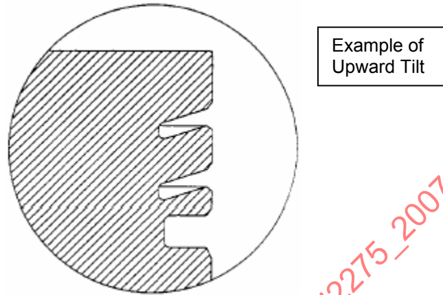
FIGURE 8 - EXAMPLE OF RADIAL UPWARD TILT (ALSO "INCLINATION")
