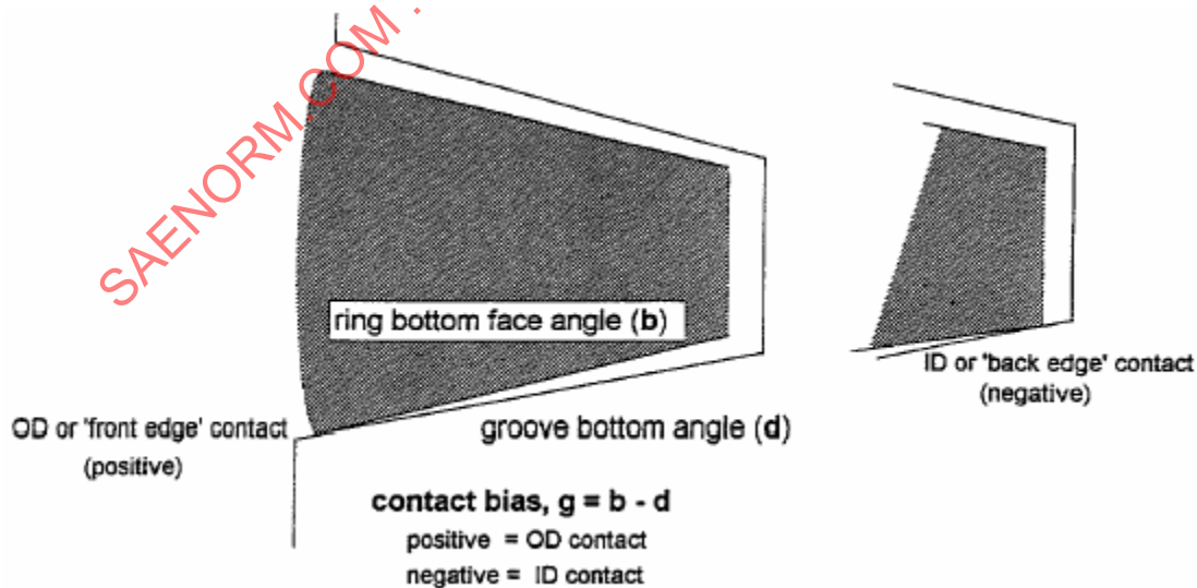
FIGURE 23 - KEYSTONE RING-TO-GROOVE CONTACT BIAS
