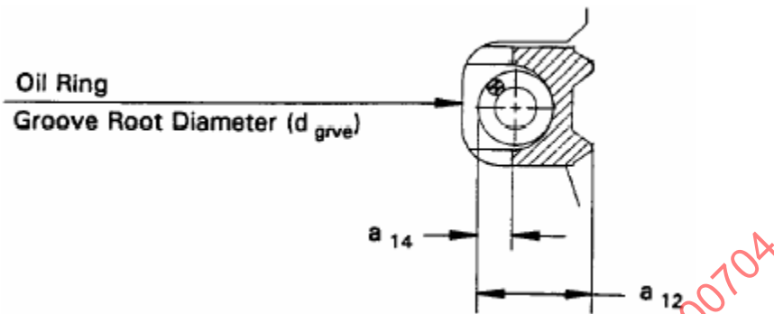
FIGURE 25 - COIL SPRING LOADED OIL RING
