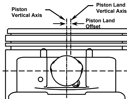
FIGURE 15 - LAND OFFSET
