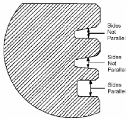
FIGURE 13 - RING GROOVE SIDE PARALLELISM
