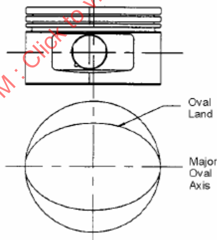
FIGURE 17 - LAND OVALITY
