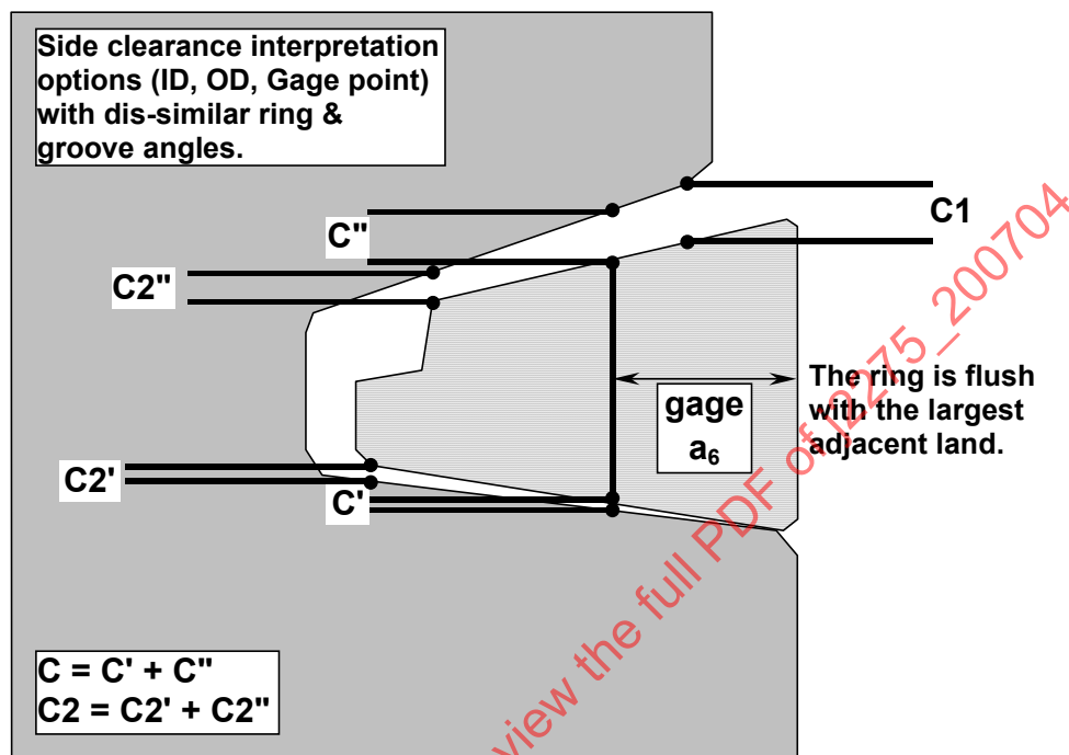
FIGURE 20 - KEYSTONE RING-TO-GROOVE CLEARANCE
