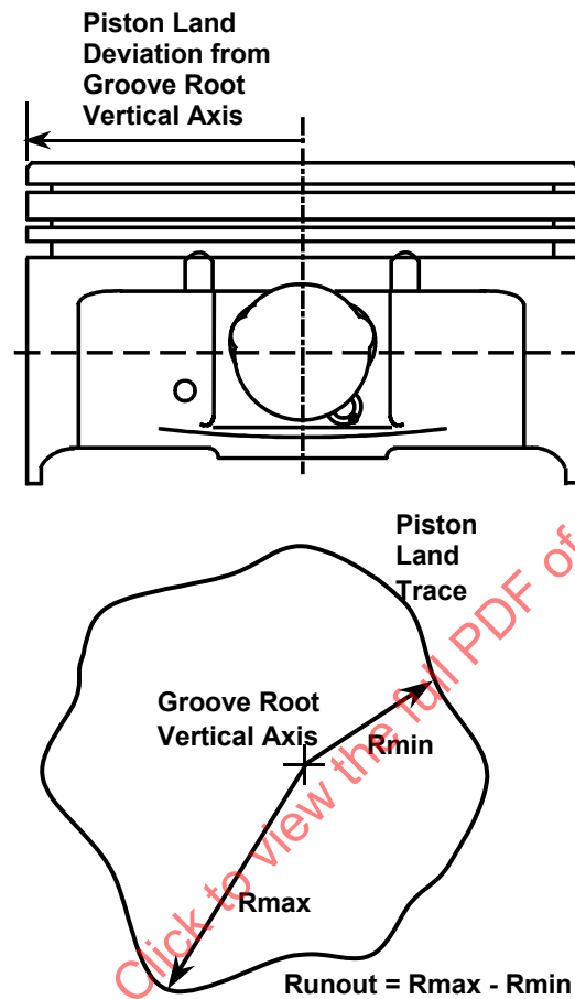
FIGURE 12 - GROOVE ROOT TO LAND RUNOUT
