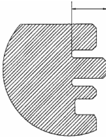
FIGURE 10 - RING GROOVE DEPTH
