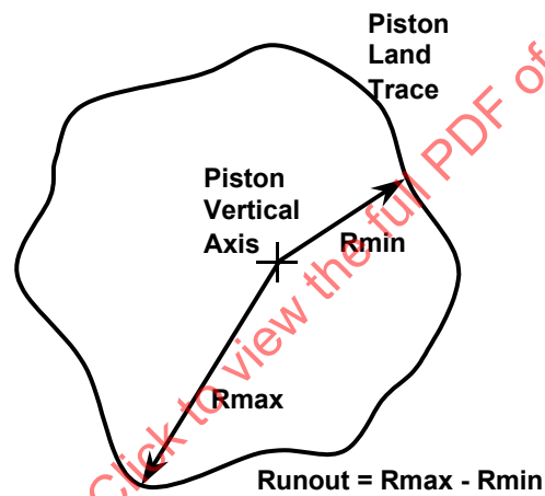
FIGURE 14 - LAND RUNOUT
