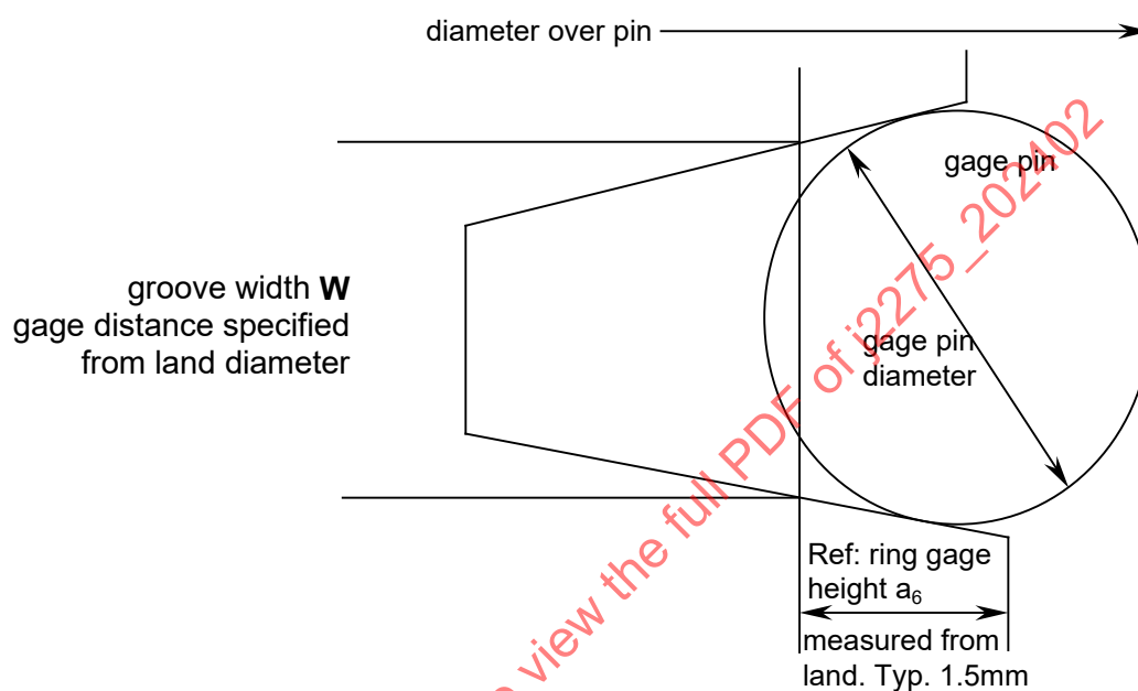
Figure 18 - Keystone groove width definition
