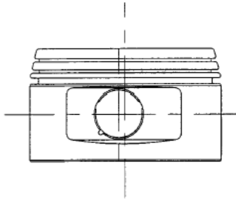
Figure 16 - Land profile
