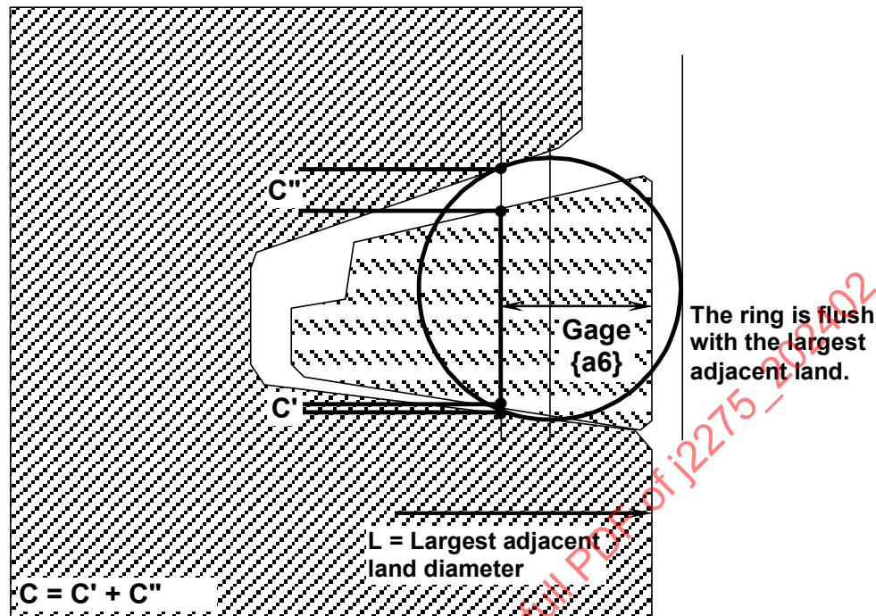
Figure 20 - Keystone ring groove clearance (example calculation)
