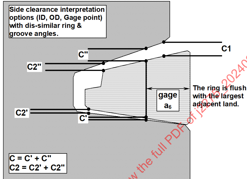
Figure 19 - Keystone ring-to-groove clearance
