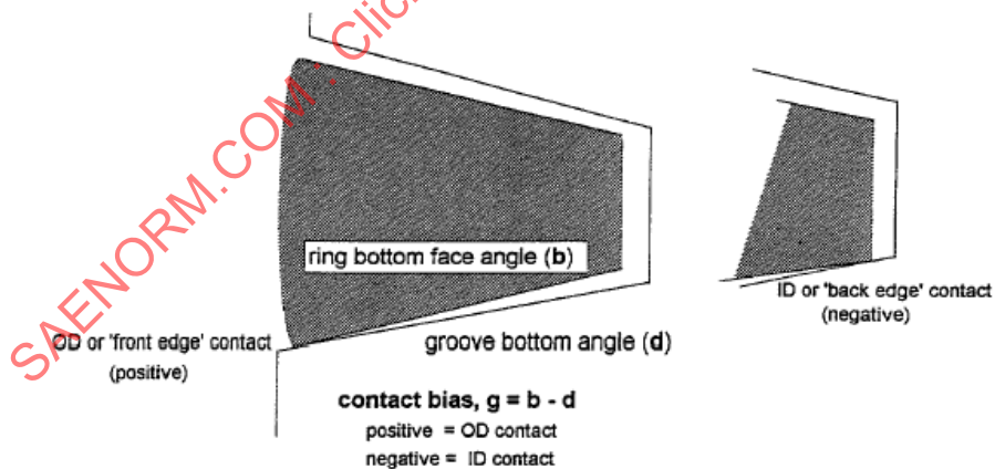
Figure 22 - Keystone ring-to-groove contact bias
