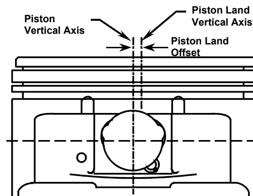
Figure 15 - Land offset
