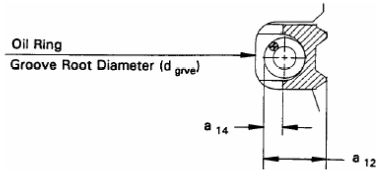
Figure 24 - Coil-spring-loaded oil ring
