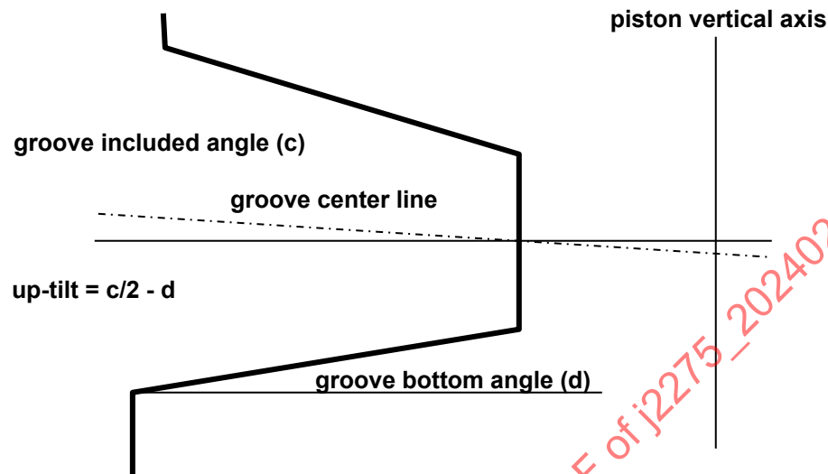
Figure 21 - Keystone groove up-tilt
