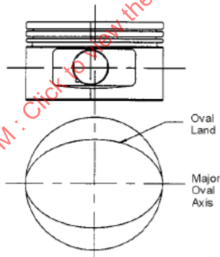
Figure 17 - Land ovality
