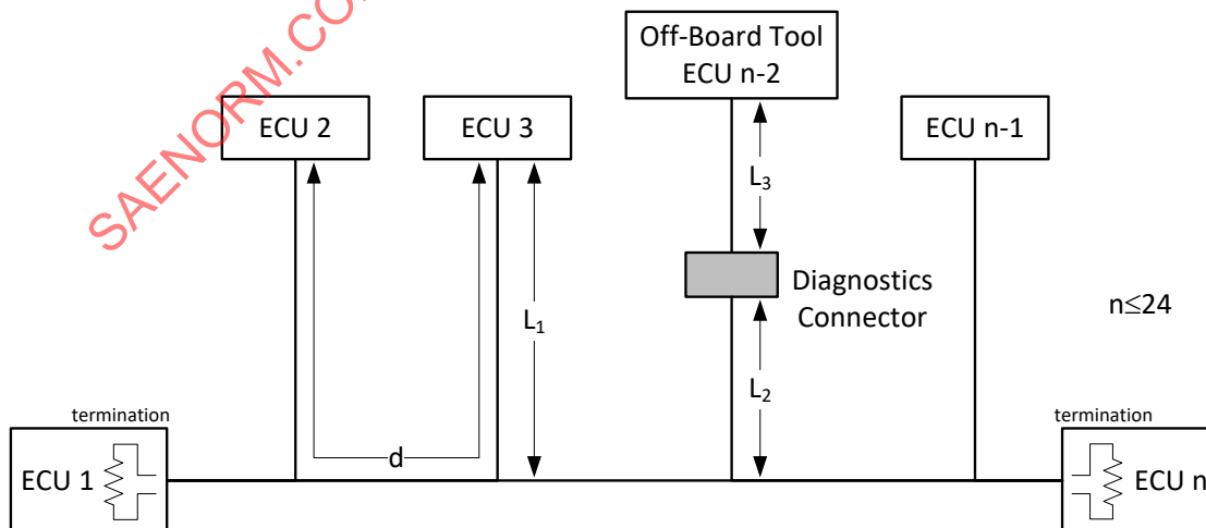
Figure 2 - Multiple on-board ECU configuration
