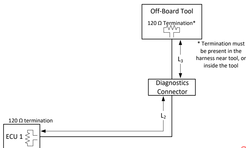
Figure 3 - Single on-board ECU configuration
