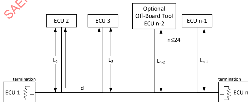
Figure 1 - Multiple on-board ECU configuration
