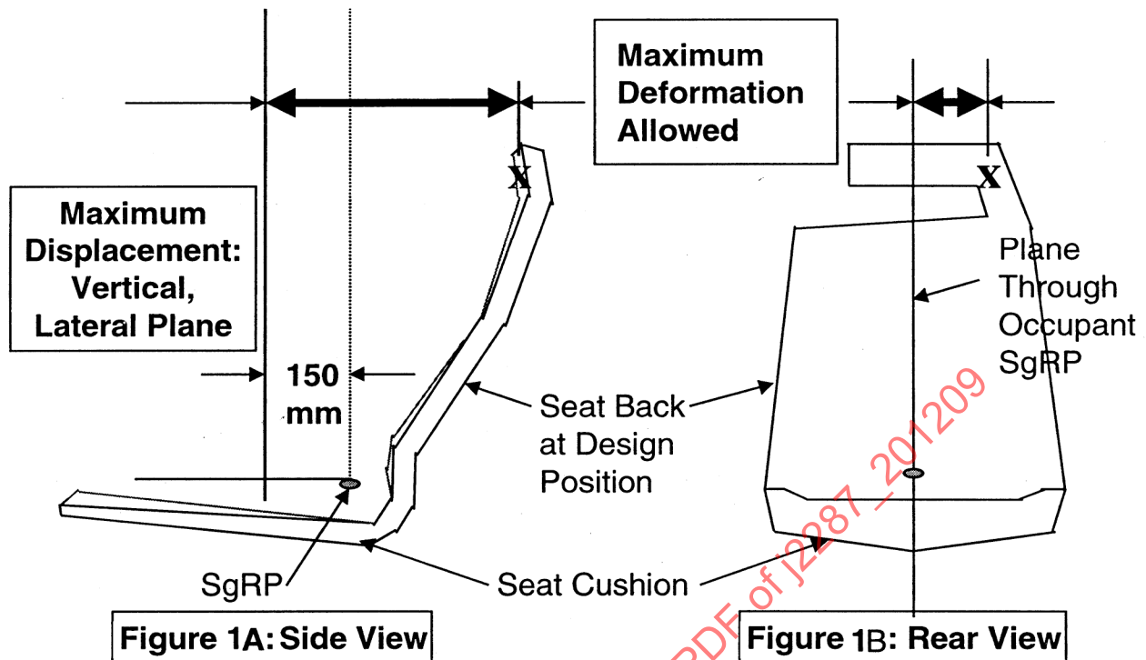
FIGURE 1—SIDE/REAR VIEWS—SEAT
