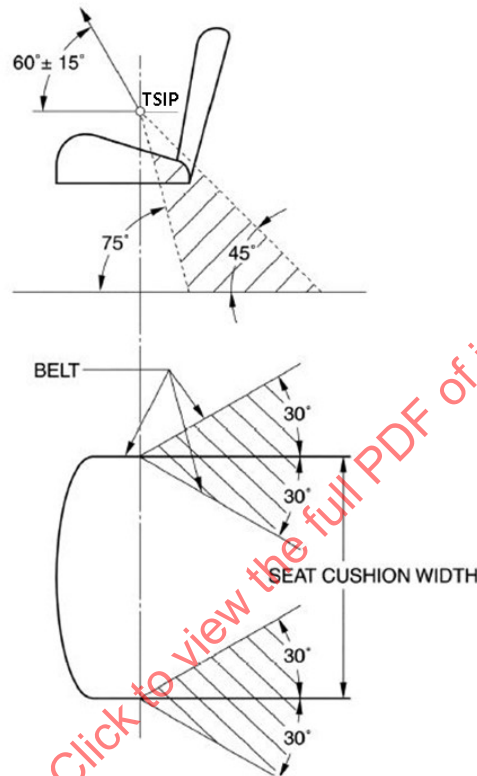
Figure 3 - Location of seat belt anchorage for pelvic portion of a type 2 and type 2a seat belt system with respect to seat index point
