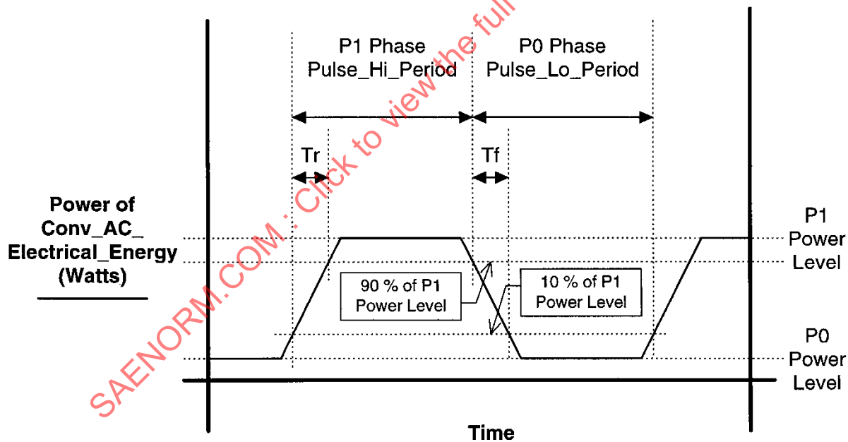
FIGURE 11 - AC-TO-AC CONVERSION PULSE MODE TIMING
