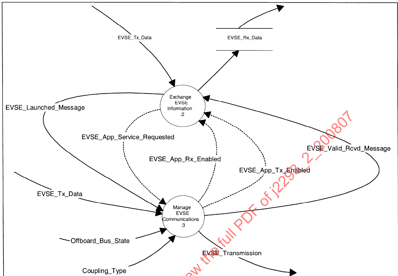
FIGURE 11 - TRANSCIVE EVSE INFORMATION DFD
