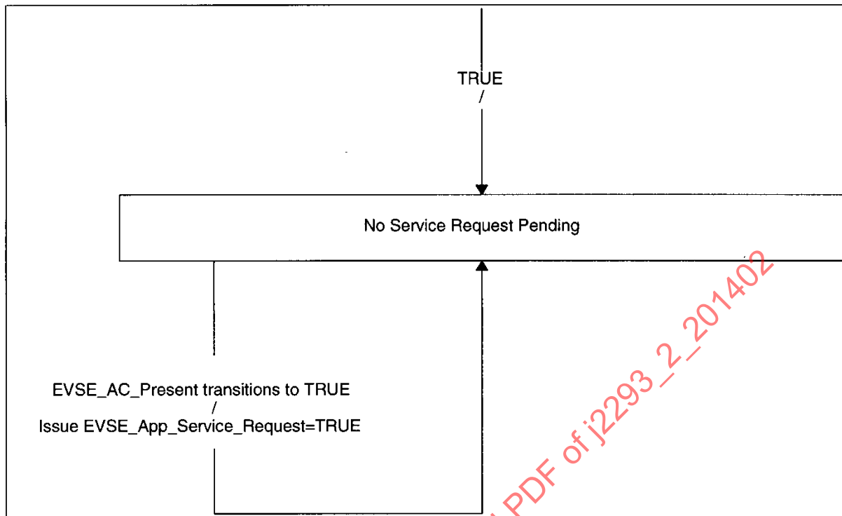
FIGURE 13 - APPLICATION SERVICE REQUEST STD
