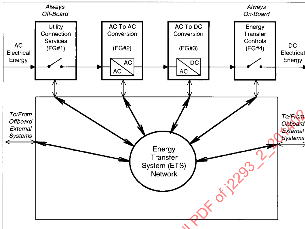
FIGURE 5 - ILLUSTRATION OF ETS NETWORK CONTEXT
