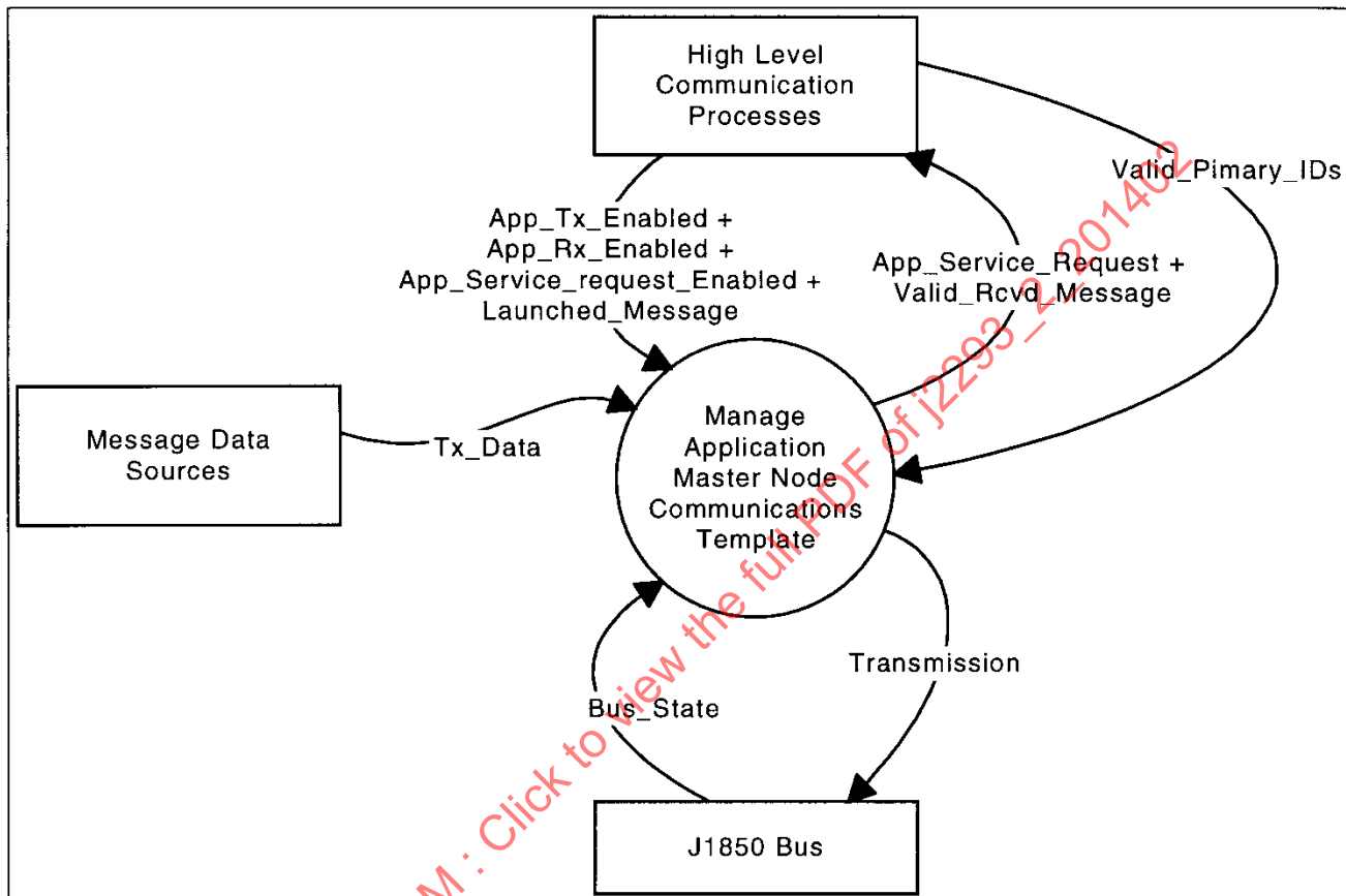
FIGURE 36 - MANAGE APPLICATION MASTER NODE COMMUNICATION CONTEXT DIAGRAM
