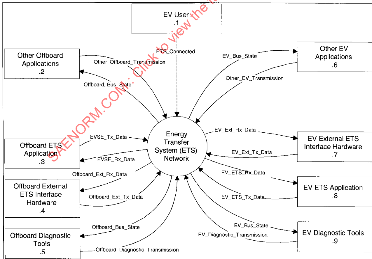
FIGURE 8 - ETS NETWORK FUNCTIONAL CONTEXT DIAGRAM
