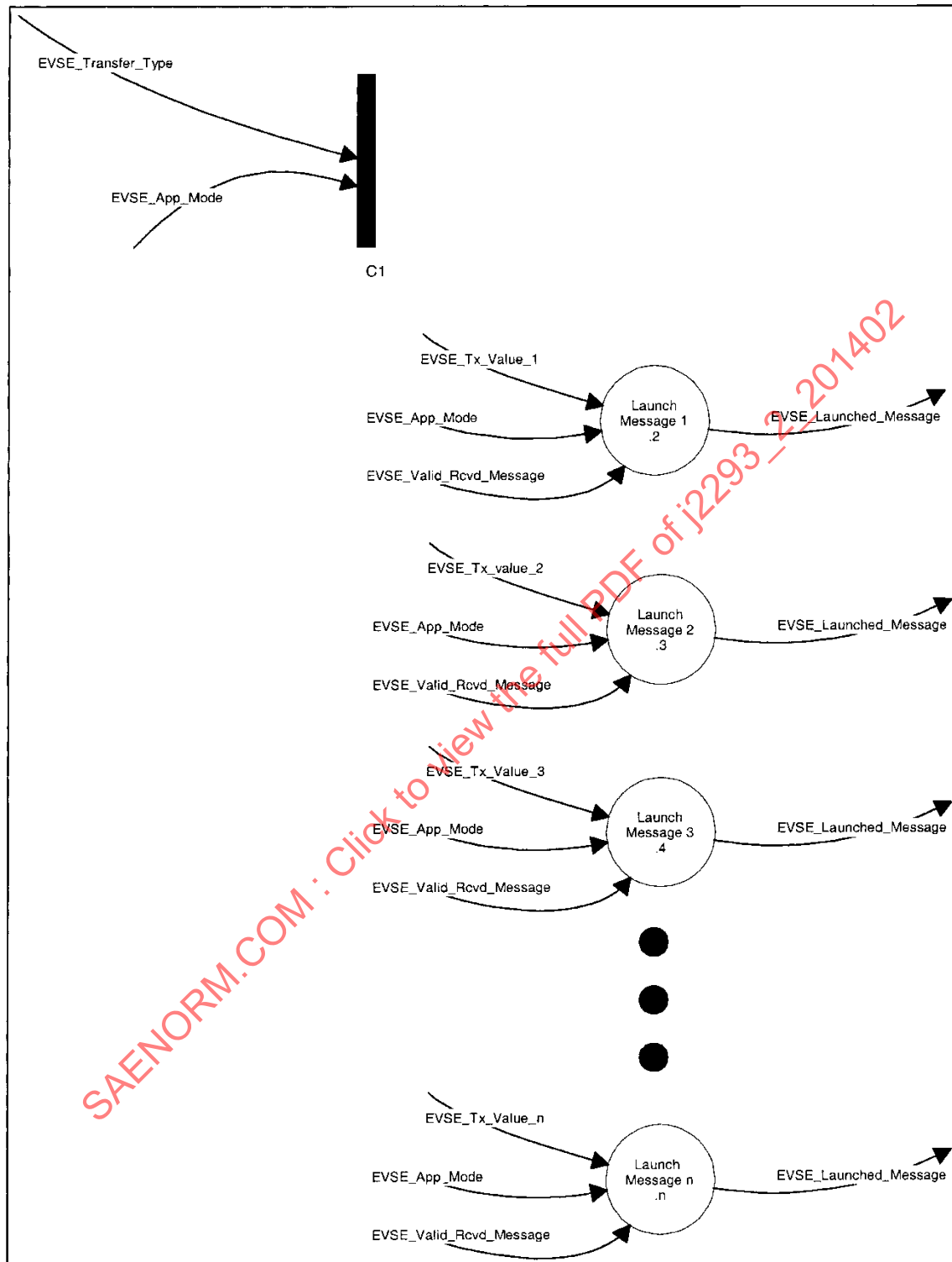
FIGURE 14 - ILLUSTRATION OF LAUNCH EVSE APPLICATION MESSAGES DFD
