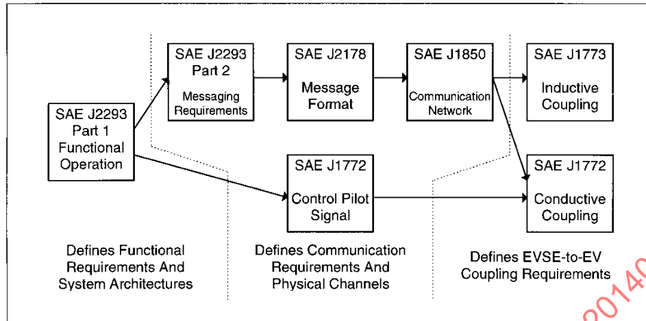
FIGURE 4 - SAE J2293 DOCUMENT INTERRELATIONSHIP
