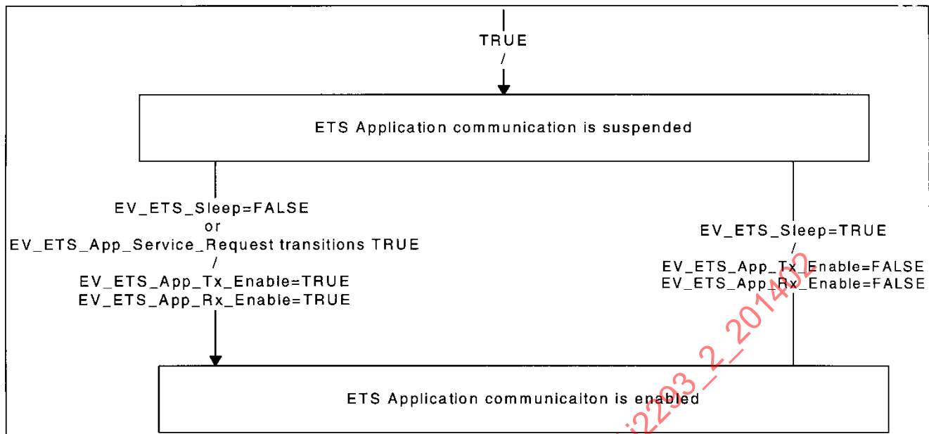
FIGURE 25 - EV ETS COMM STATE STD
