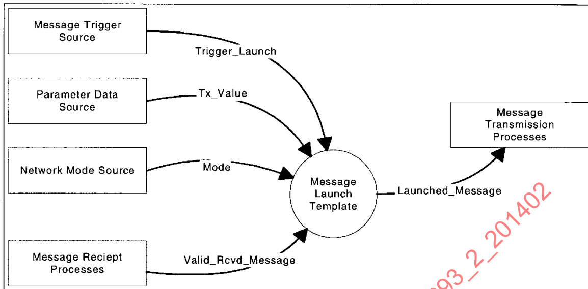
FIGURE 42 - LAUNCH MESSAGE TEMPLATE FUNCTIONAL CONTEXT
