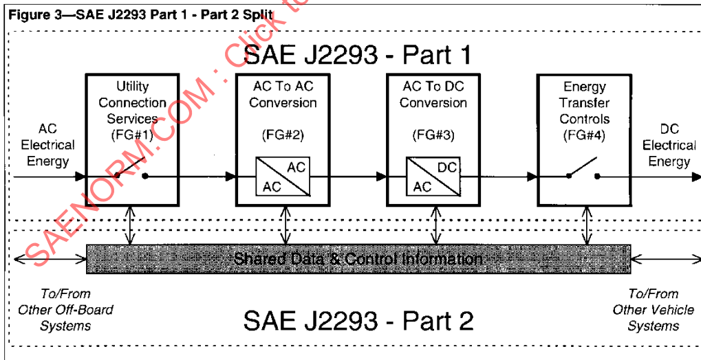
FIGURE 3 - SAE J2293 PART 1 - PART 2 SPLIT
