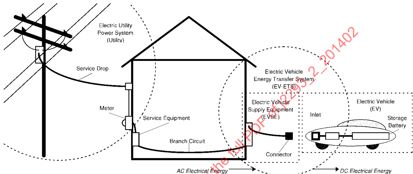
FIGURE 1 - ELECTRIC VEHICLE ENERGY TRANSFER SYSTEM PHYSICAL CONTEXT
