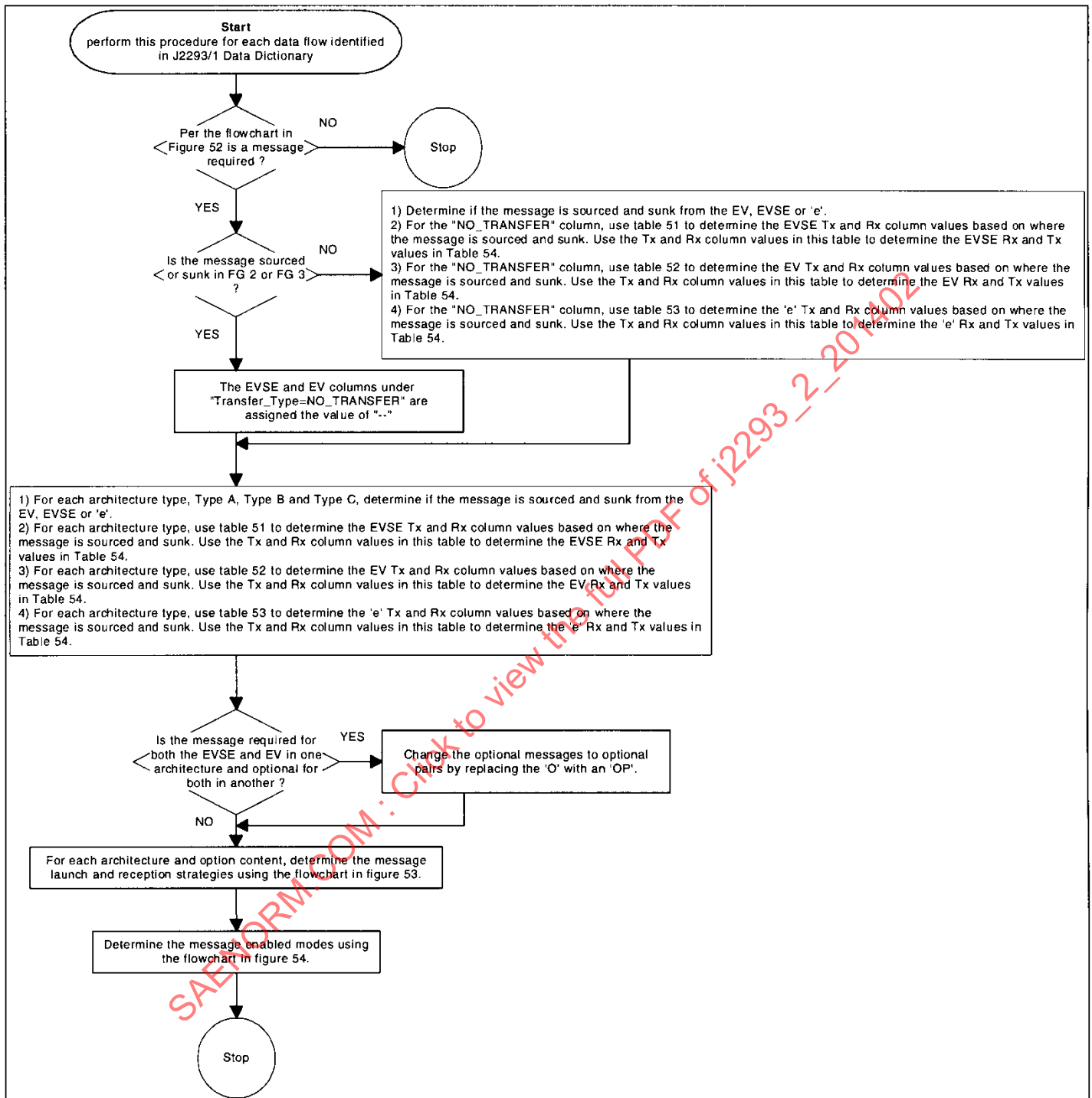
FIGURE 52 - FLOWCHART FOR CREATING MESSAGE TABLES
