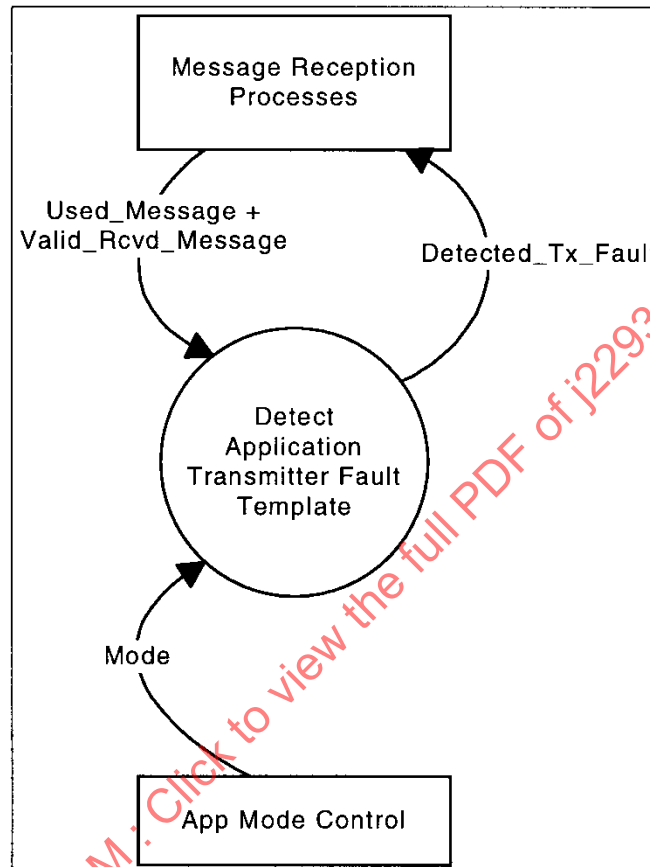
FIGURE 39 - DETECT APPLICATION TRANSMITTER FAULT TEMPLATE CONTEXT DIAGRAM
