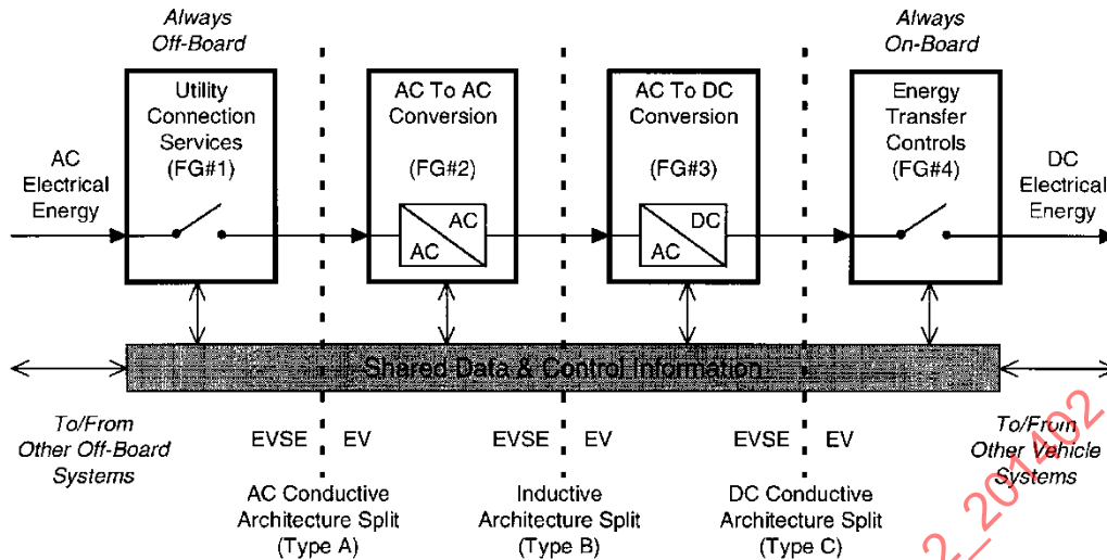
FIGURE 2 - EV ETS FUNCTIONAL GROUP SERIES ENERGY CONVERSION
