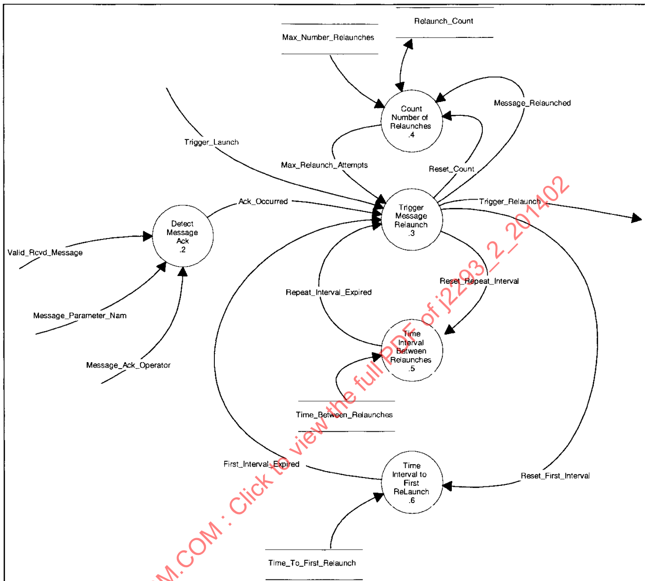
FIGURE 46 - RELAUNCH MESSAGE DFD
