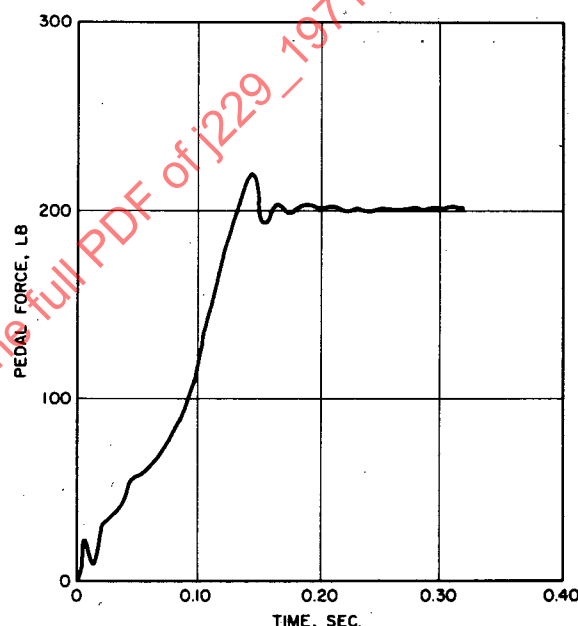
FIG. 1—TYPICAL SPIKE BRAKE APPLICATION
