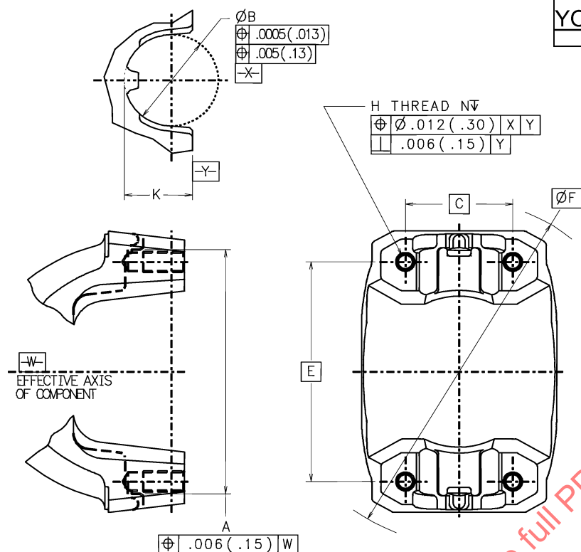
FIGURE 1—HALF ROUND EARWORK YOKE DIMENSION STANDARD (See Table 3)
