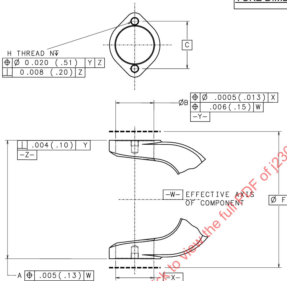
FIGURE 2—FULL ROUND EARWORK YOKE DIMENSION STANDARD (See Table 4)
