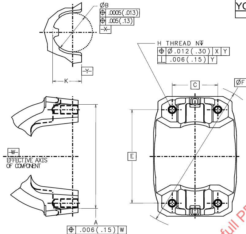
Figure 1 - Half round earwork yoke dimensions standard (see Table 3)
