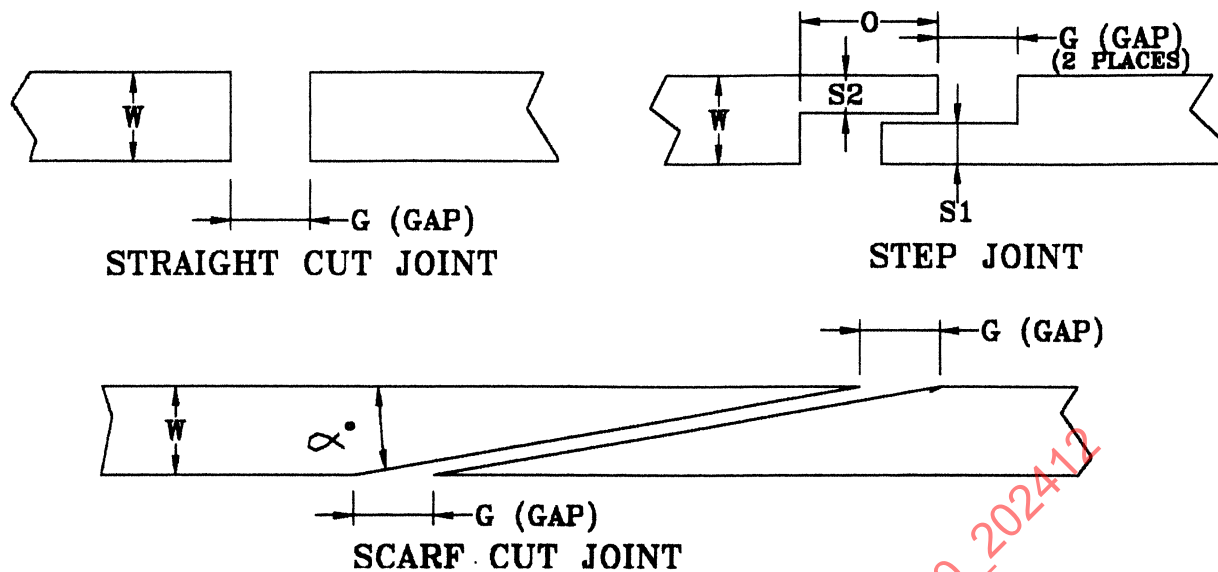
Figure 7 - Joint details
