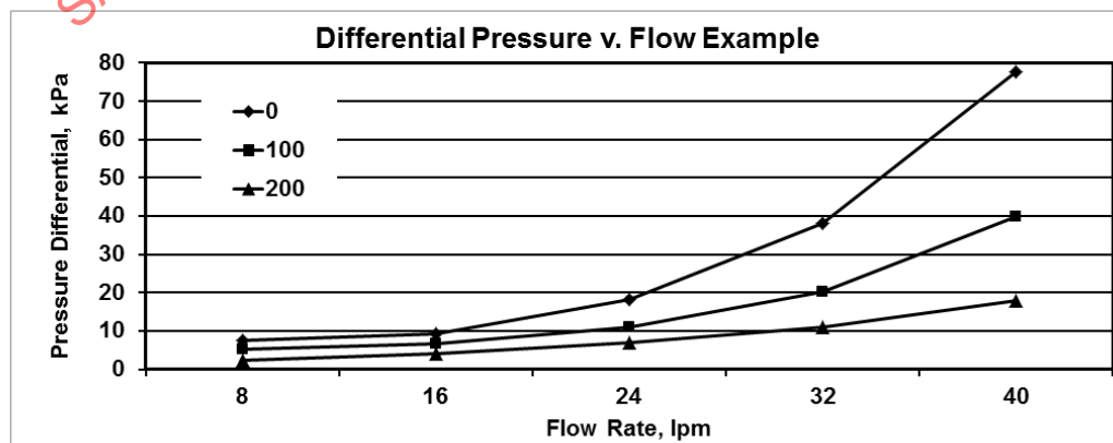
FIGURE 6 - FILTER DESIGN/APPLICATION DATA SHEET
