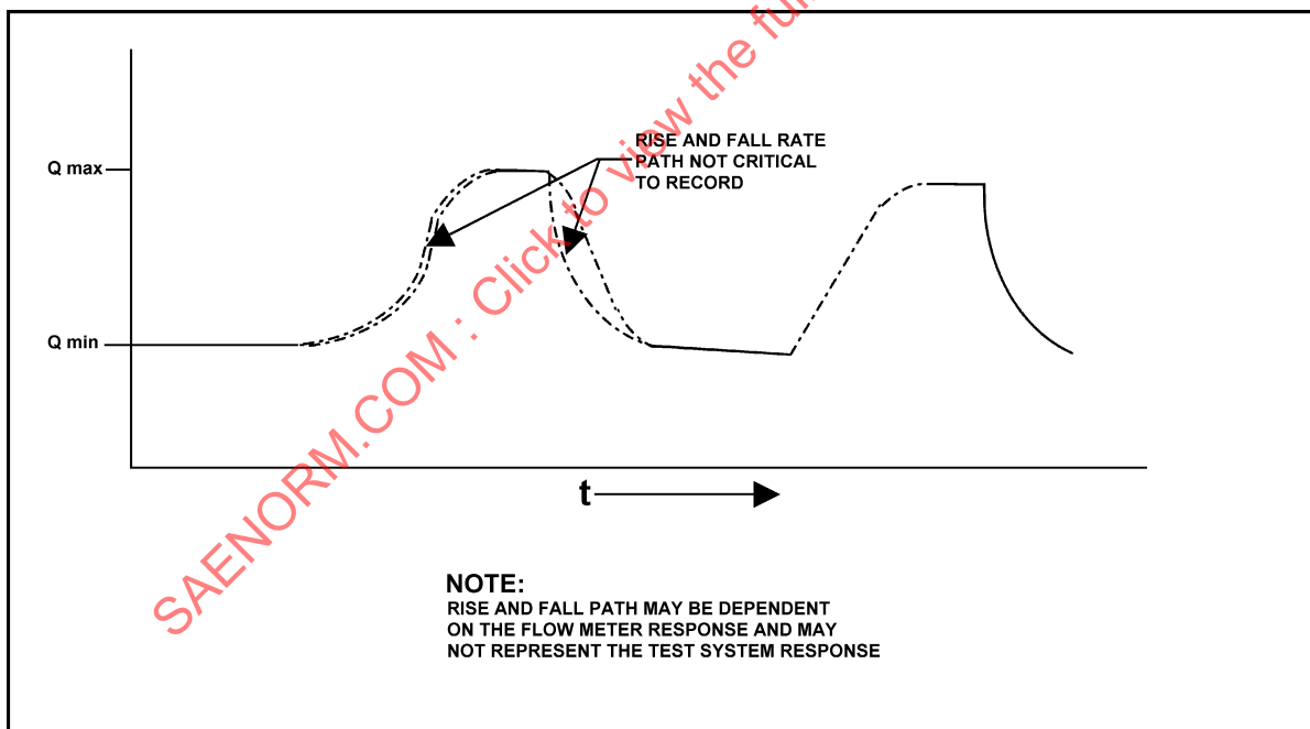
FIGURE 7B - PULSED FLOW EFFICIENCY TEST: TYPICAL PULSED FLOW PROFILE RISE AND FALL RATE GUIDANCE
