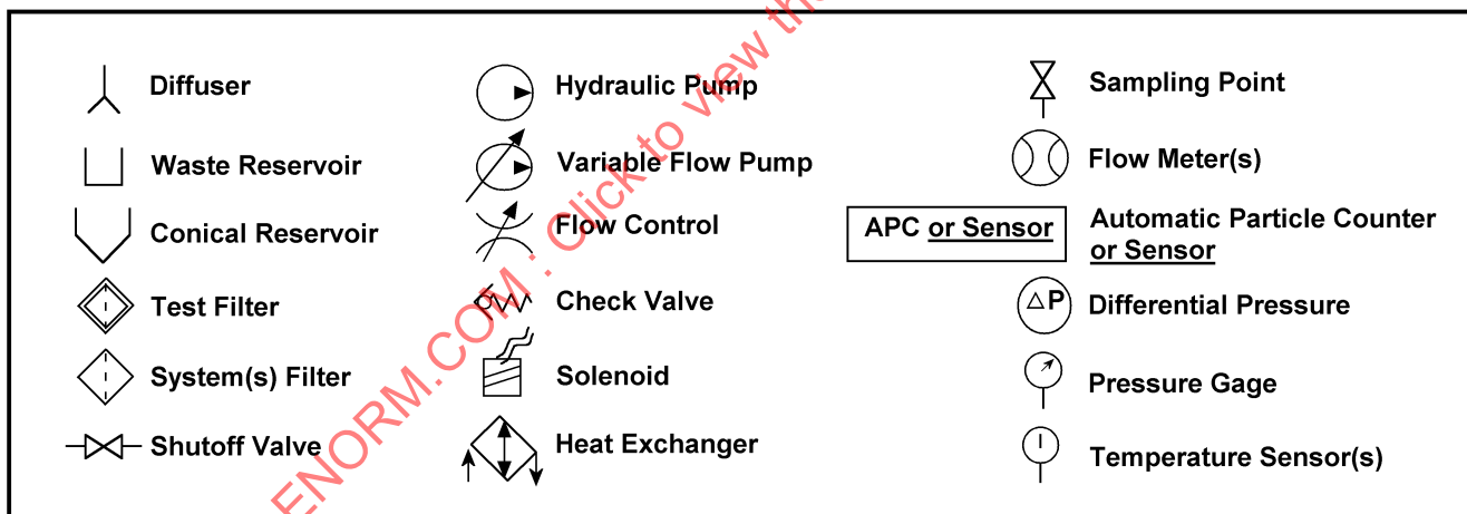
FIGURE 3 - HYDRAULIC SCHEMATIC LEGEND
