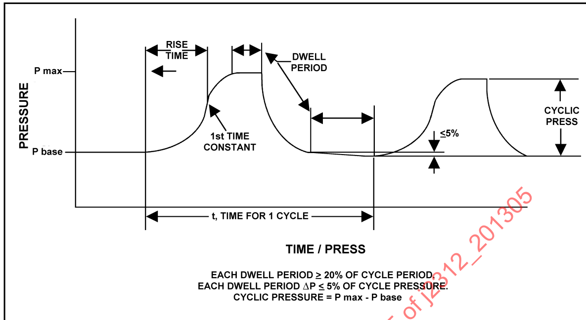
FIGURE 7A - PULSED FLOW EFFICIENCY TEST: TYPICAL PULSED FLOW PROFILE
