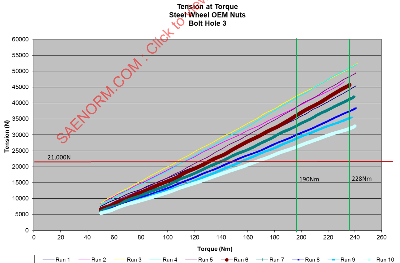
Figure 2 - Example of tension at torque bolt hole graph
