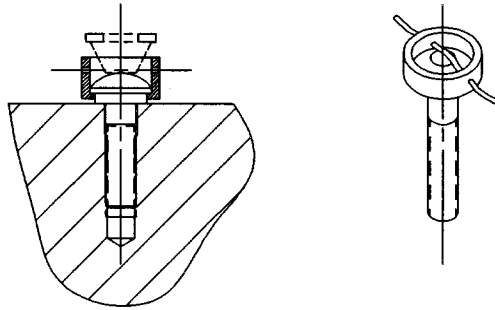
FIGURE 3—BREAKAWAY CAPSCREW
