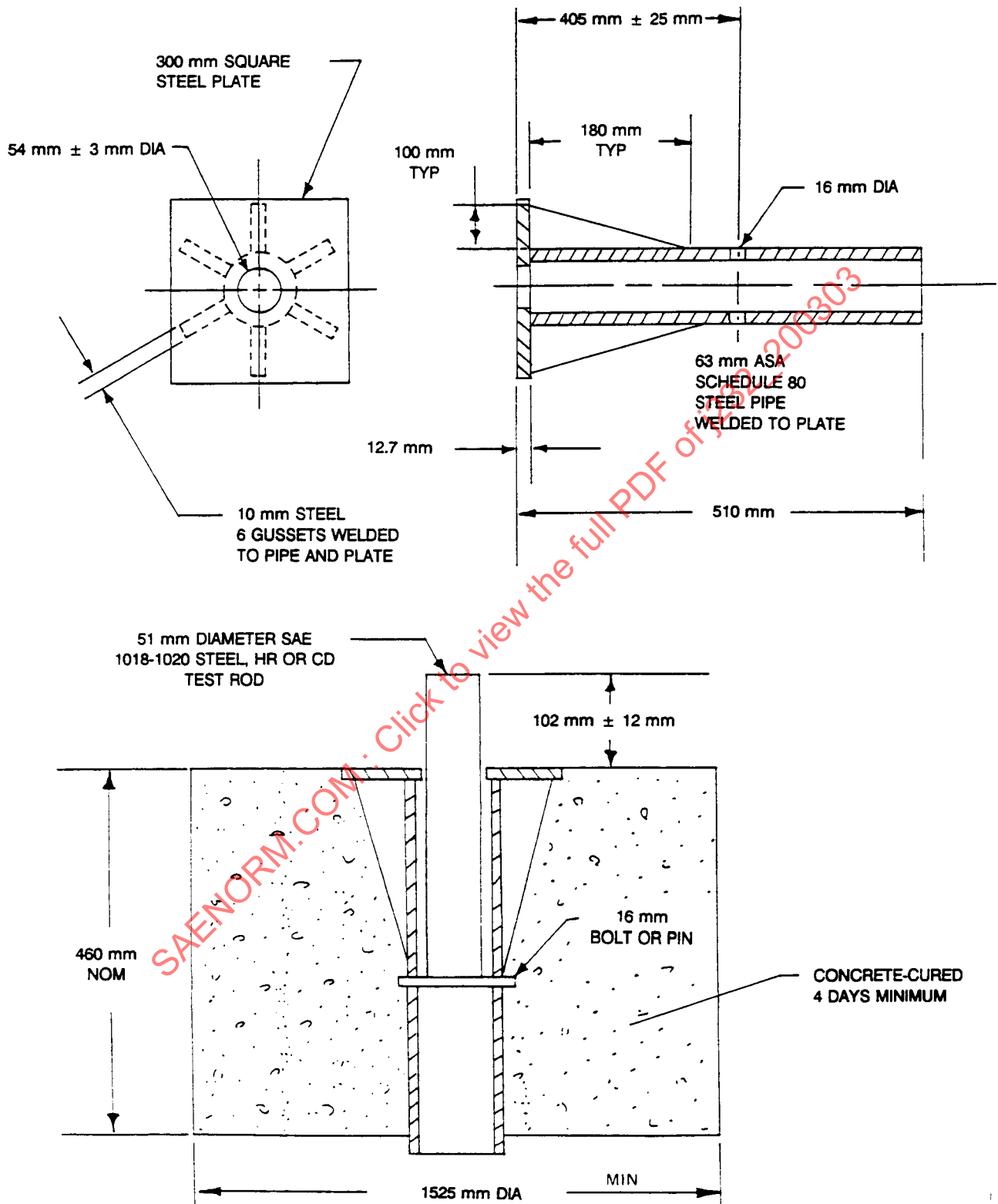
FIGURE 8A—IMPACT TEST FIXTURE
