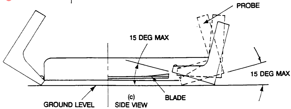
FIGURE 6—FOOT PROBE
