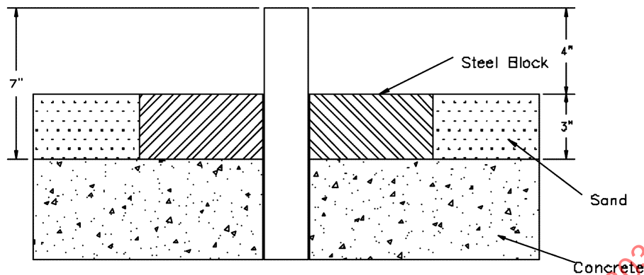
FIGURE 8B—SAND BASE IMPACT TEST FIXTURE
