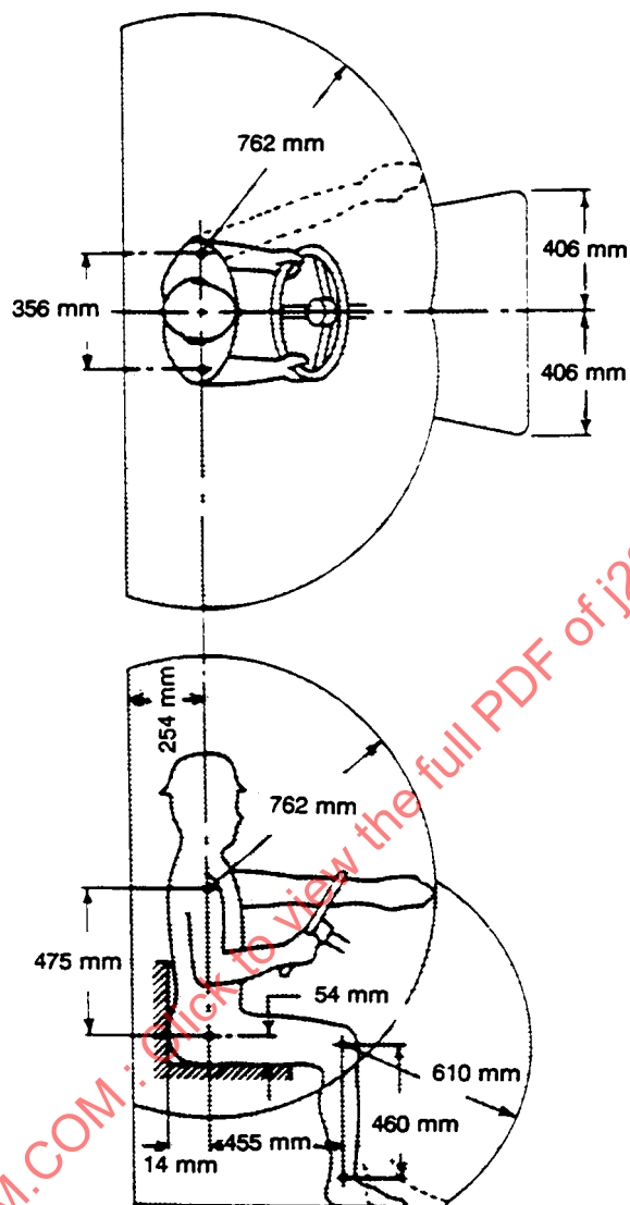
FIGURE 1—OPERATOR ZONE
