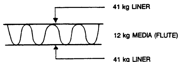
FIGURE 4—SINGLE WALL
