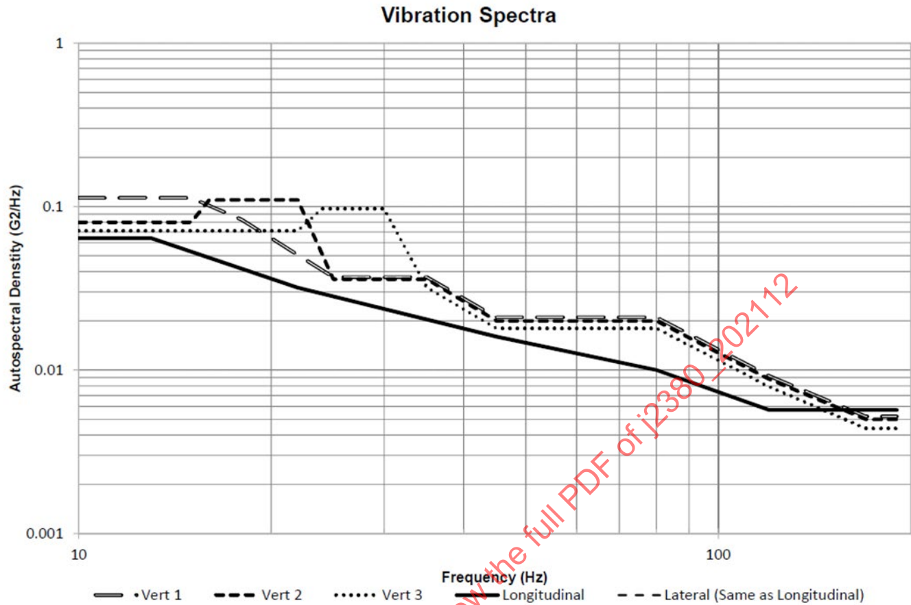
Figure 2 - Vibration spectra for random vibration test
