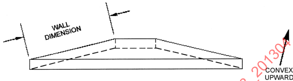
FIGURE 2—CONICAL WASHER TOLERANCE
