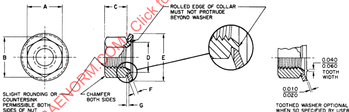
FIGURE 1—NUT AND CONICAL SPRING WASHER ASSEMBLY
