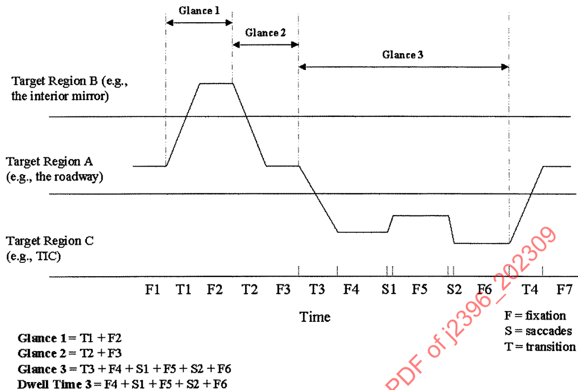
Figure 2 - Chronological relationship of driver visual allocation between and within AOIs*
