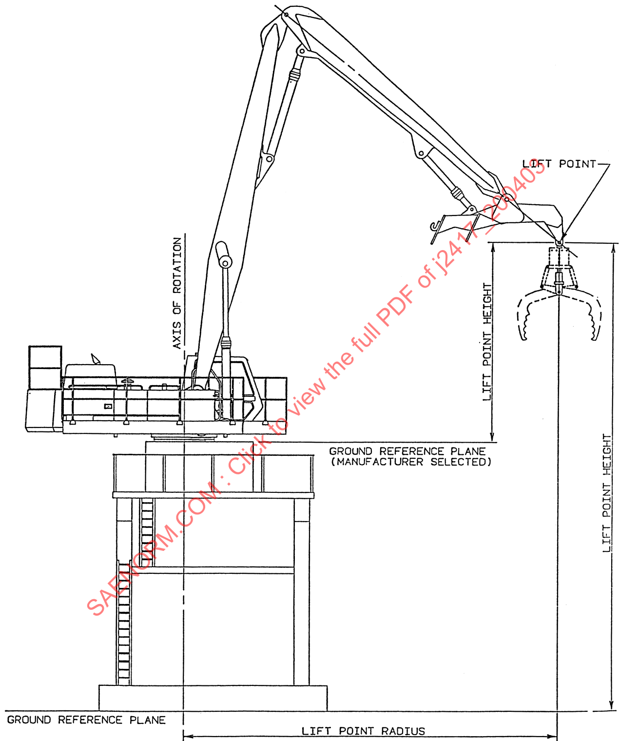
FIGURE 6—PEDESTAL-MOUNTED LOG LOADER
