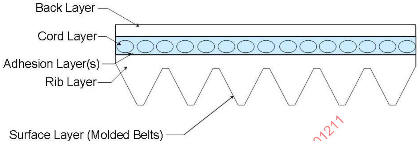
FIGURE 1 - BELT CROSS-SECTION
