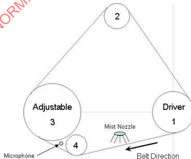
FIGURE 6 - NOISE TEST STAND CONFIGURATION
