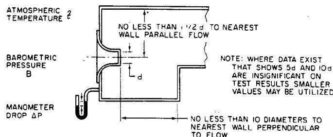
FIGURE 2 - Nozzle Discharging From Atmosphere Into a Vessel
