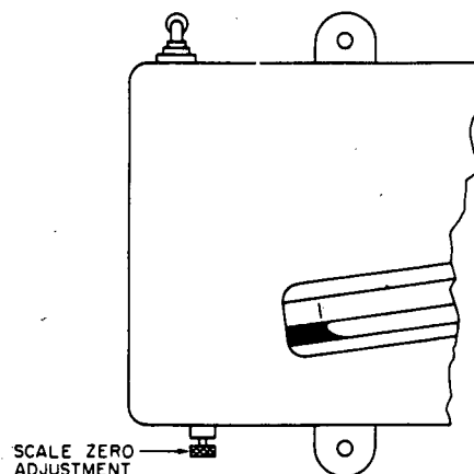
FIGURE 9 - Inclined Manometer Adjustment
