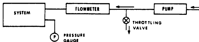
FIGURE 6 - Installation for Measuring Leak Rate
