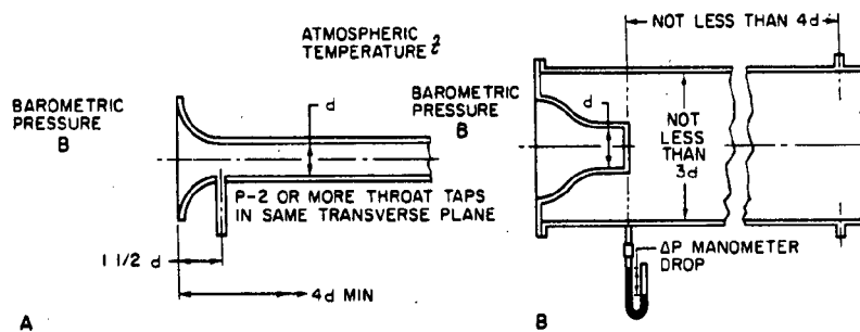
FIGURE 3 - Nozzle Discharging From Atmosphere Into a Pipe
