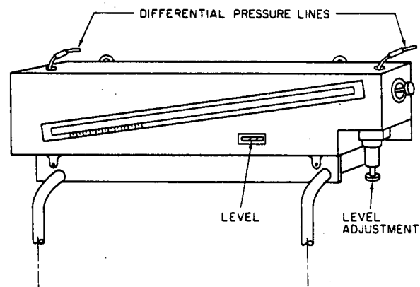
FIGURE 7 - Inclined Manometer Adjustment
