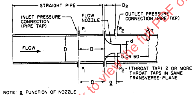
FIGURE 4 - Nozzle in a Pipe
