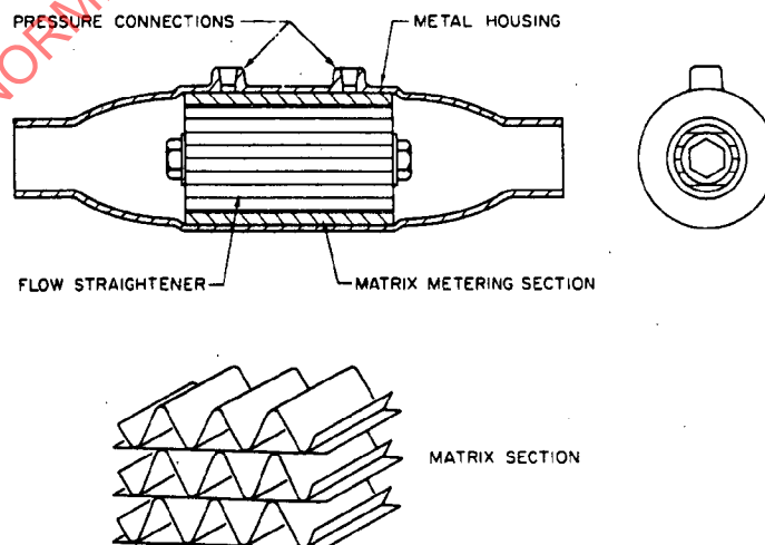
FIGURE 5 - General Construction of Laminar Flow Element
