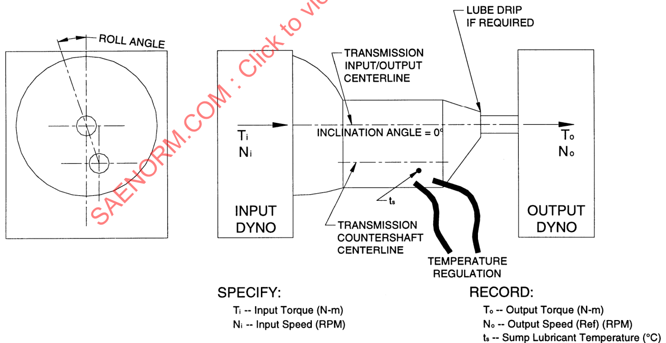
FIGURE 2—TYPICAL RWD MANUAL TRANSMISSION DYNAMOMETER SCHEMATIC
