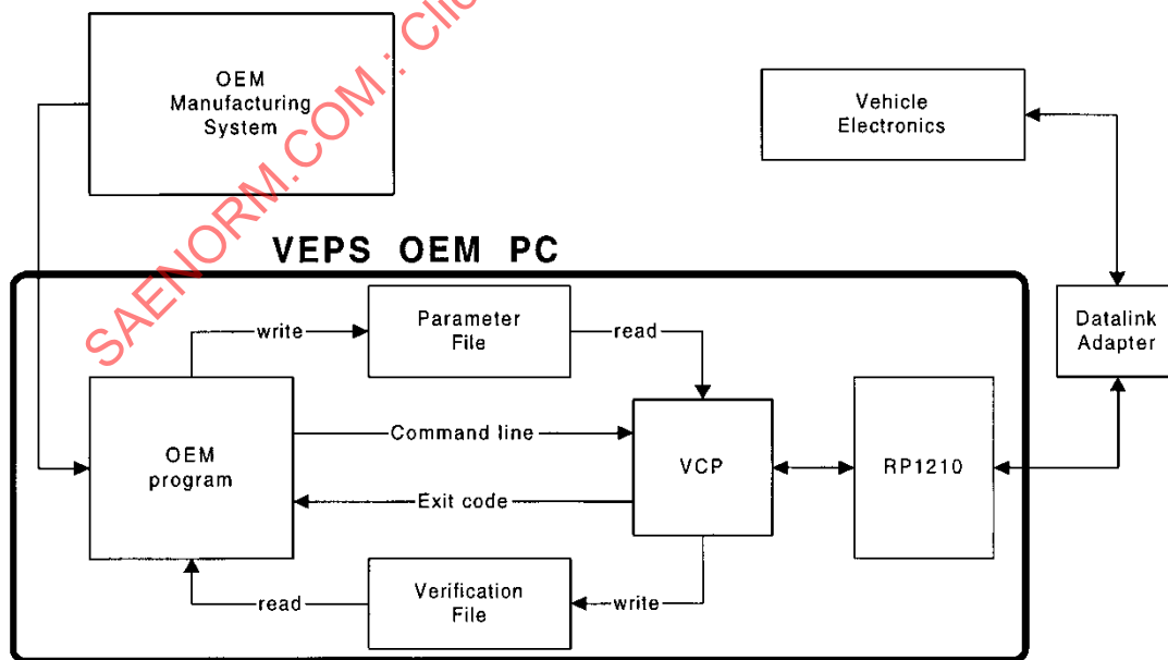
FIGURE 2 - VEPS COMPONENTS AND INTERFACES
