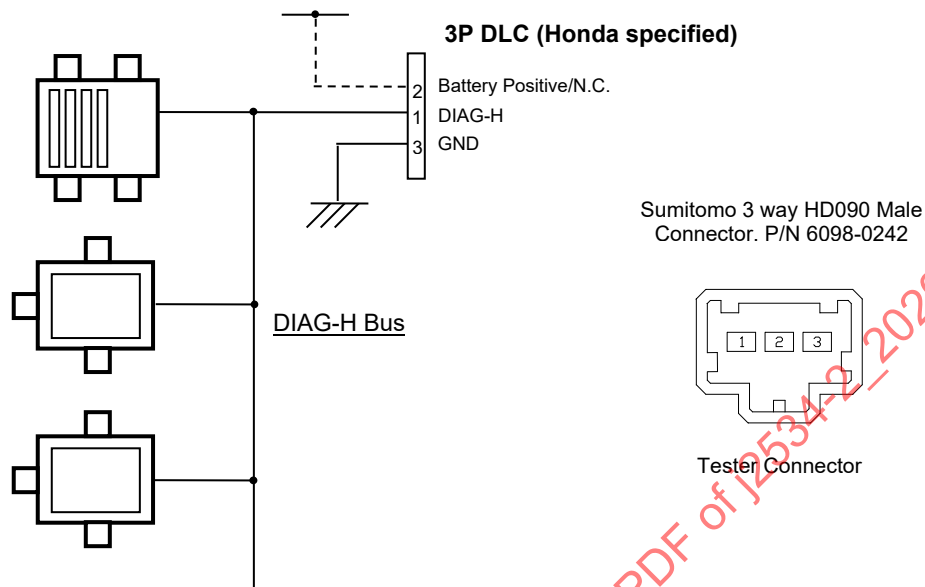
Figure 6 - Diagnostic communication line configuration (3-pin DLC model)
