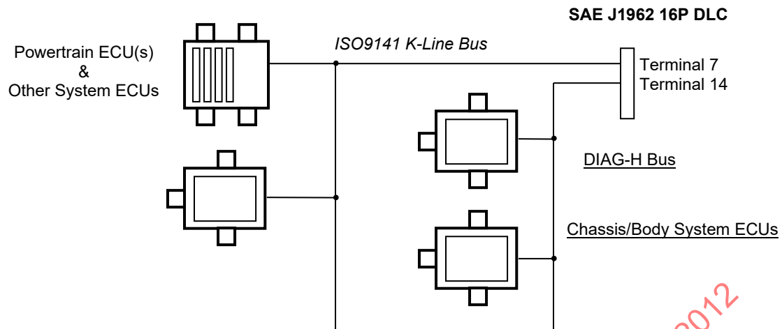
Figure 8 - Diagnostic communication line configuration (16-pin DLC model without CAN)
