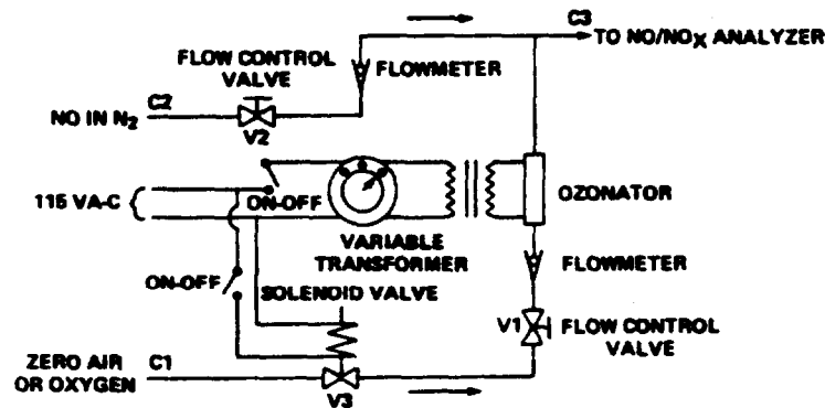
FIGURE 8—NO x GENERATOR FOR CONVERTER EFFICIENCY DETERMINATION
