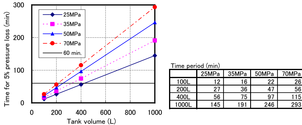
FIGURE A12 - TIME PERIODS FOR 5% PRESSURE LOSS
