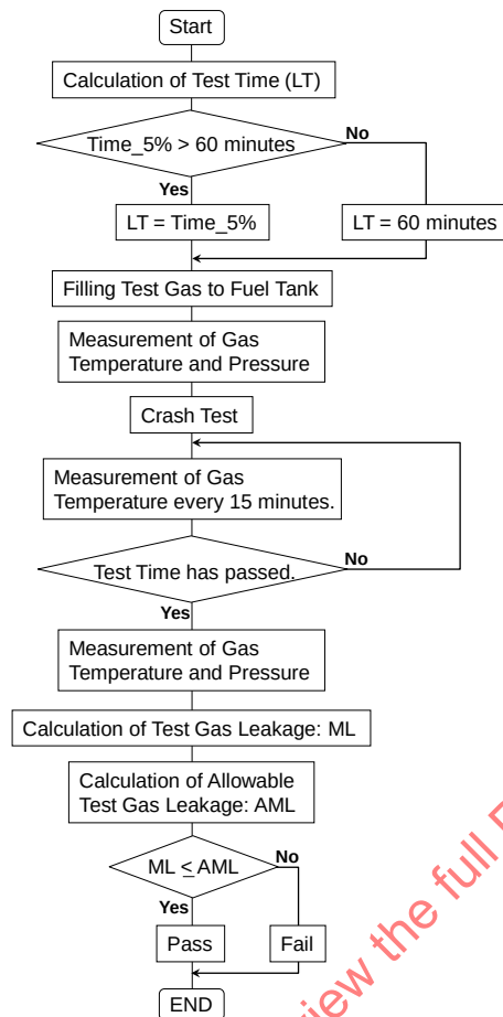
FIGURE A4 - TEST PROCEDURE
