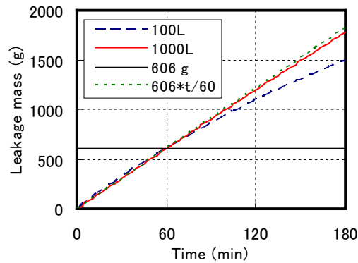
FIGURE A6 – LEAKAGE MASS CHARACTERISTICS OVER TIME
