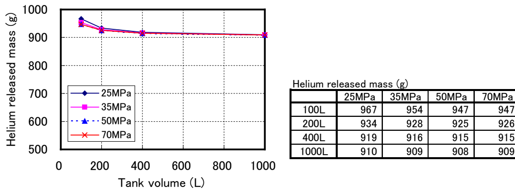
FIGURE A9 - HELIUM LEAKAGE OVER 60 MINUTES
