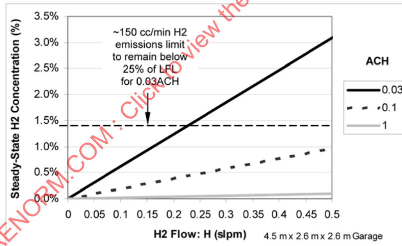
FIGURE C1 - CALCULATED STEADY-STATE HYDROGEN CONCENTRATIONS VS HYDROGEN EMISSION RATE FOR VARIOUS AIR EXCHANGE RATES WITH STANDARD ENCLOSURE
