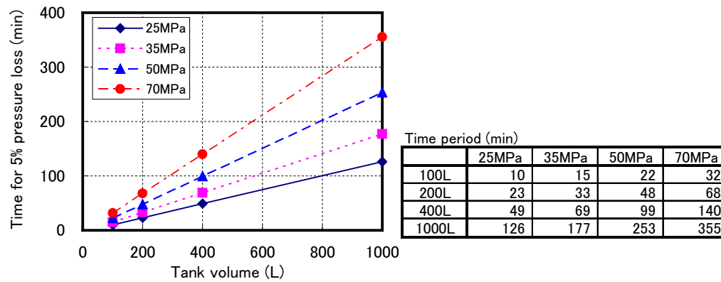
FIGURE A14 - TIME PERIODS FOR 5% PRESSURE LOSS
