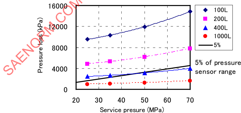
FIGURE A2 - PRESSURE LOSS WITH 606 g HYDROGEN LEAKAGE
