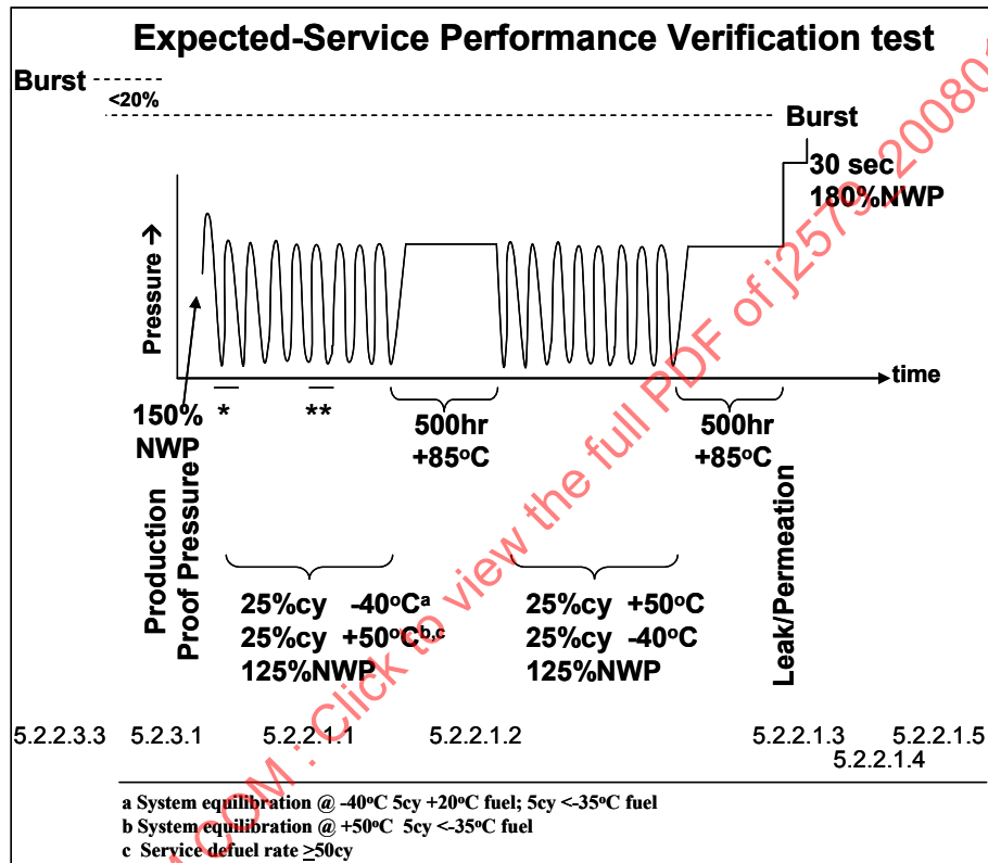
FIGURE 4 COMPRESSED HYDROGEN STORAGE EXPECTED-SERVICE PERFORMANCE VERIFICATION
