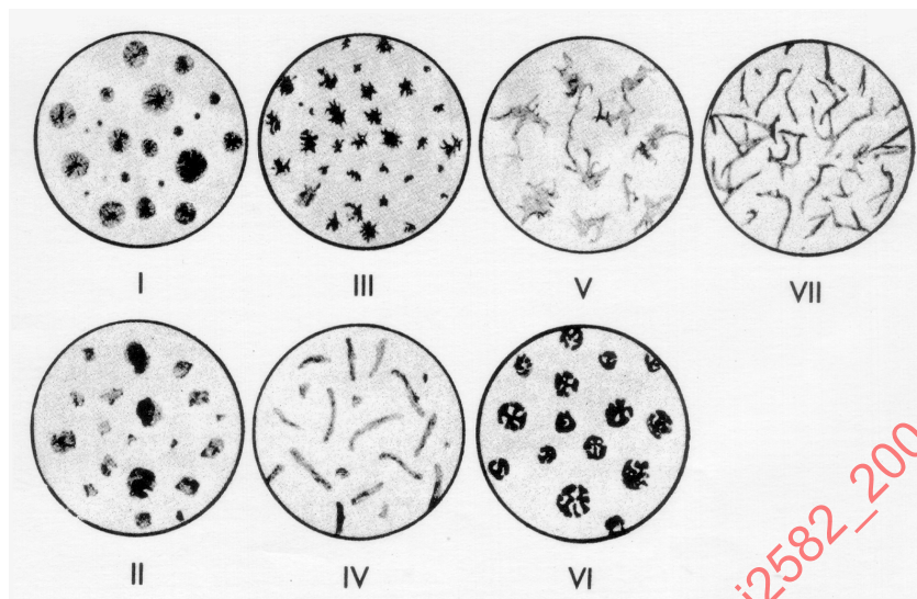
FIGURE 1—CLASSIFICATION OF GRAPHITE SHAPE IN CAST IRONS (FROM ASTM A 247)
