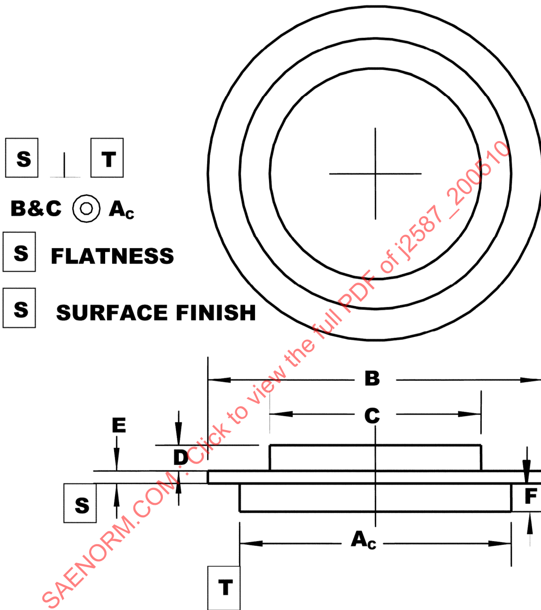
FIGURE A1—CLOSURE COVER FLANGE
