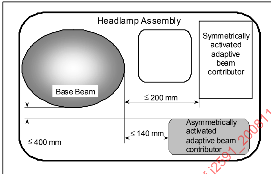
FIGURE 1 - ADAPTIVE BEAM CONTRIBUTOR SPACING HEADLAMP EXAMPLE
