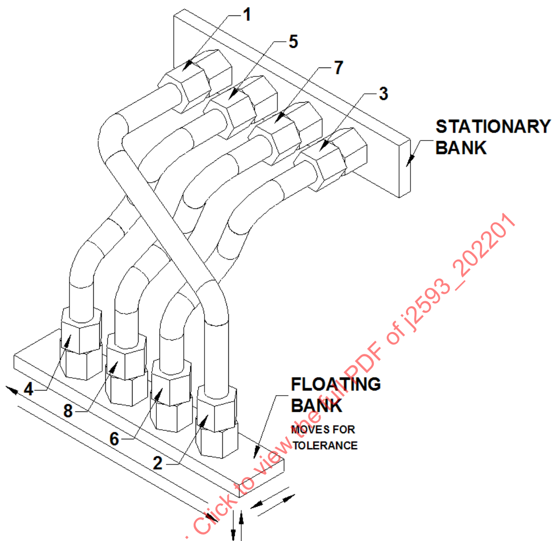
Figure 2 - Multiple tube installation tightening sequence
