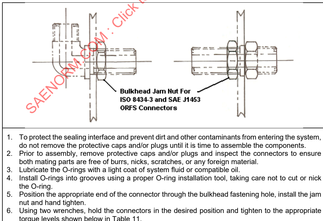
Figure 11 - ISO 8434-3 and SAE J1453 ORFS connectors recommended assembly procedures for bulkhead fastening jam nuts
