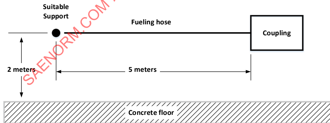
Figure 5.9.2 - Test arrangement for dropping test
