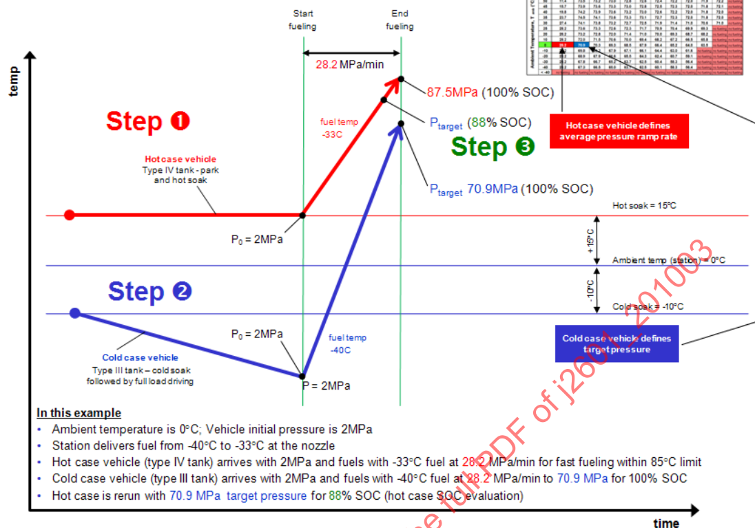
FIGURE A3 - EXAMPLE OF APPROACH USED TO GENERATE LOOK-UP TABLE VALUES
