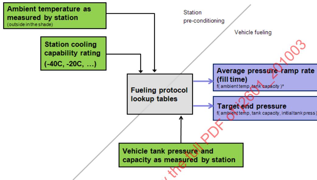
FIGURE A4 - PROCESS FLOW FOR NON-COMMUNICATION FUELING
