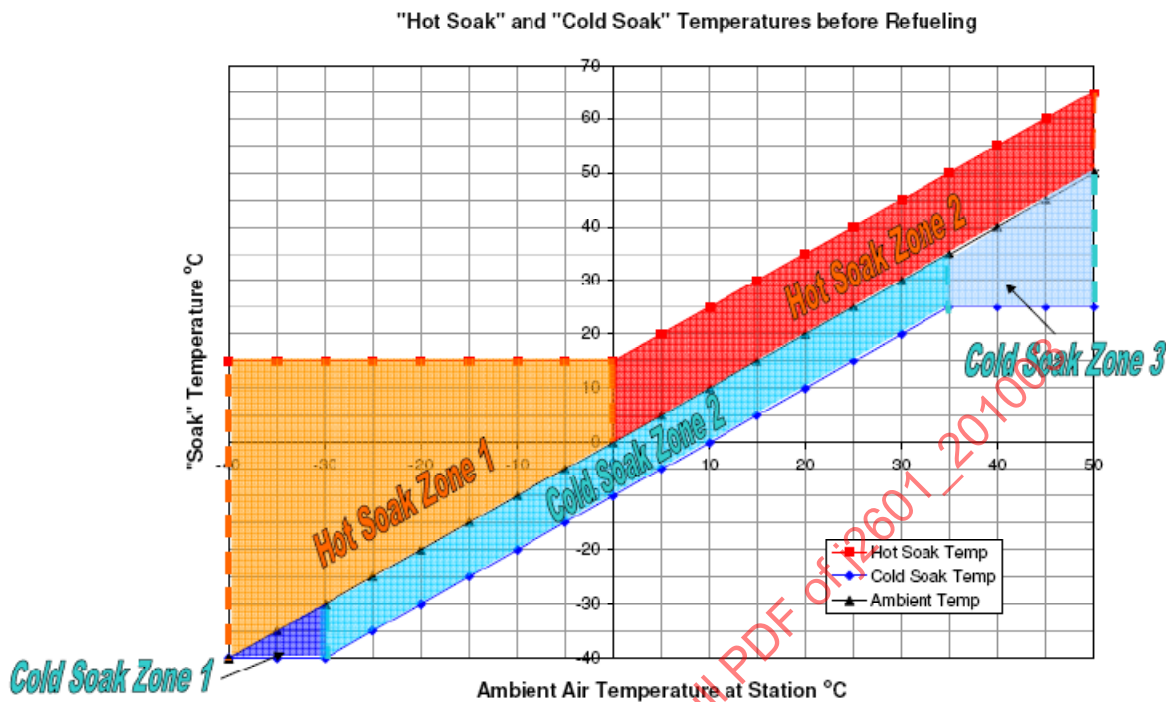
FIGURE A1 - "COLD SOAK" AND "HOT SOAK" ONBOARD STORAGE TEMPERATURES COMPARED TO AMBIENT TEMPERATURE
