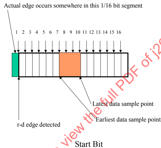
FIGURE 2—BIT SAMPLE TIMING
