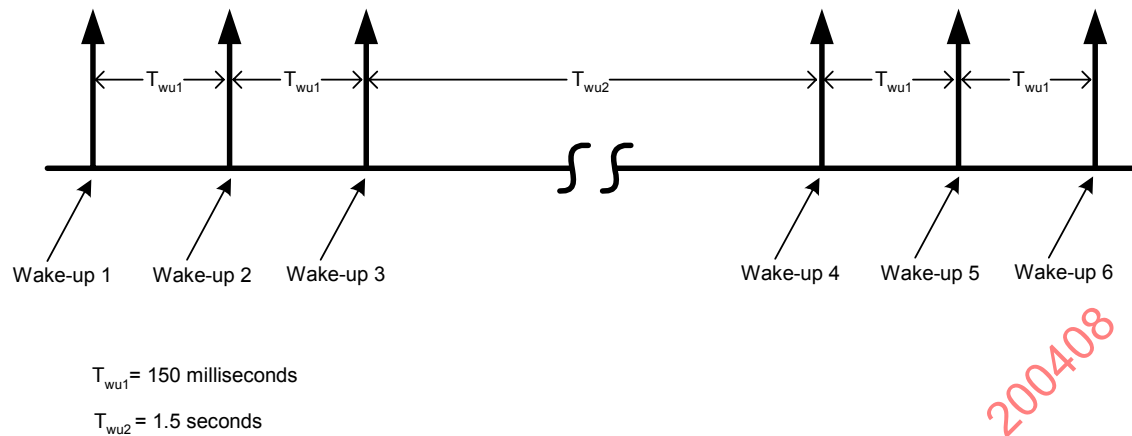
FIGURE 1—WAKE-UP SIGNAL TIMING
