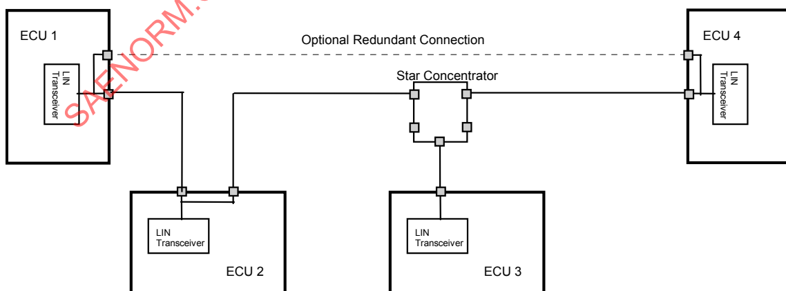
FIGURE 8—LIN COMBINATION RING AND STAR TOPOLOGY
