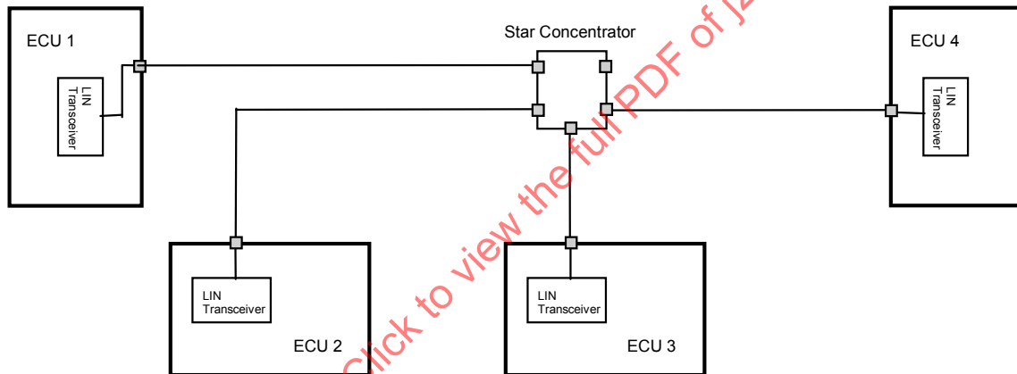
FIGURE 7—LIN STAR TOPOLOGY
