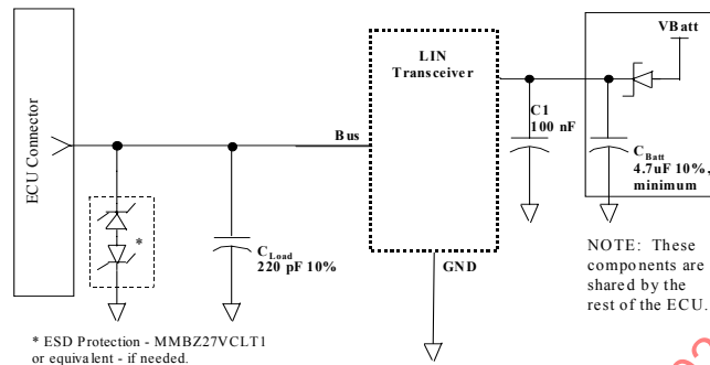
FIGURE 3—TYPICAL LIN SLAVE BUS INTERFACE
