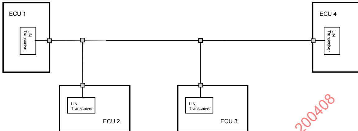
FIGURE 6—LIN LINEAR TOPOLOGY
