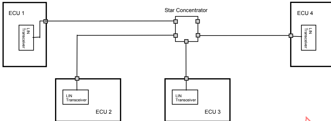
FIGURE 9 - LIN STAR TOPOLOGY
