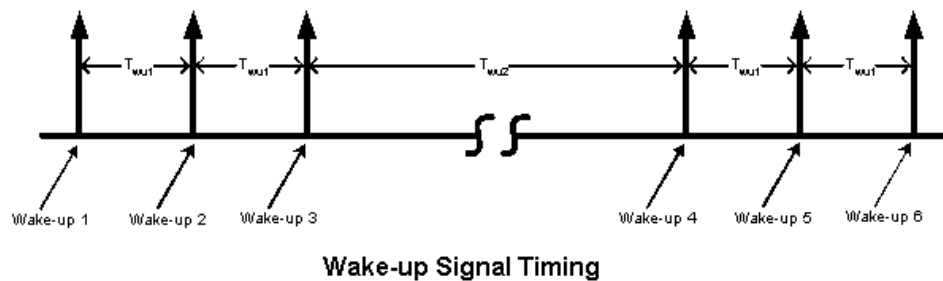
FIGURE 3 - WAKE-UP SIGNAL TIMING
