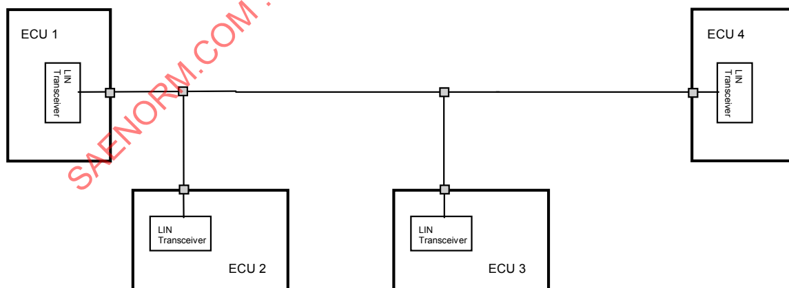
FIGURE 8 - LIN LINEAR TOPOLOGY
