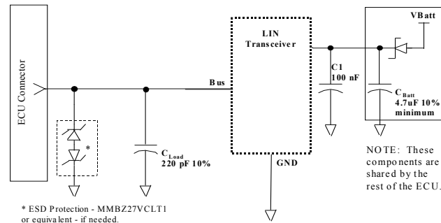
FIGURE 5 - TYPICAL LIN SLAVE BUS INTERFACE
