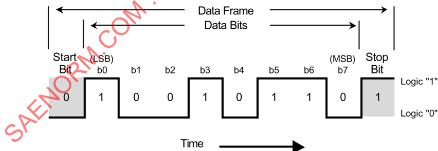
Figure 8 - This example depicts the data frame transmission of character $69
