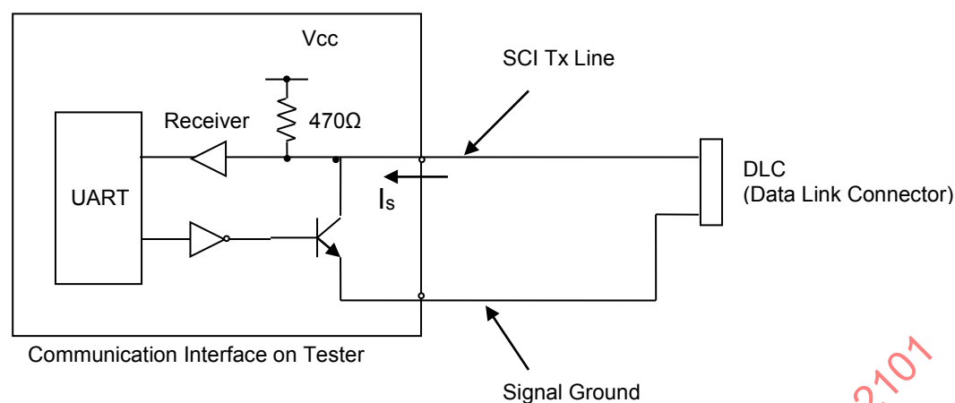
Figure 6.2 - Recommended interface circuit on tester
