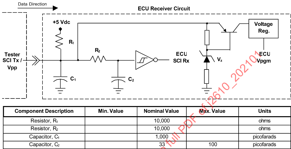
Figure 6 - Representative ECU receiver circuit with typical component values
