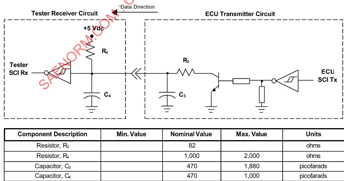
Figure 7 - Representative ECU transmitter circuit with typical component values
