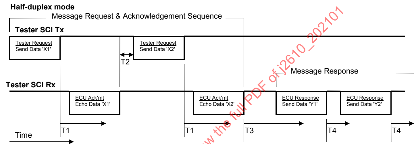
Figure 9 - Two-frame message request/acknowledgement sequence with a two-frame message response during a diagnostic session
