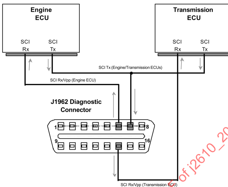
Figure 4 - Configuration 'A' depicted with single SCI line shared per pair of emission ECUs
