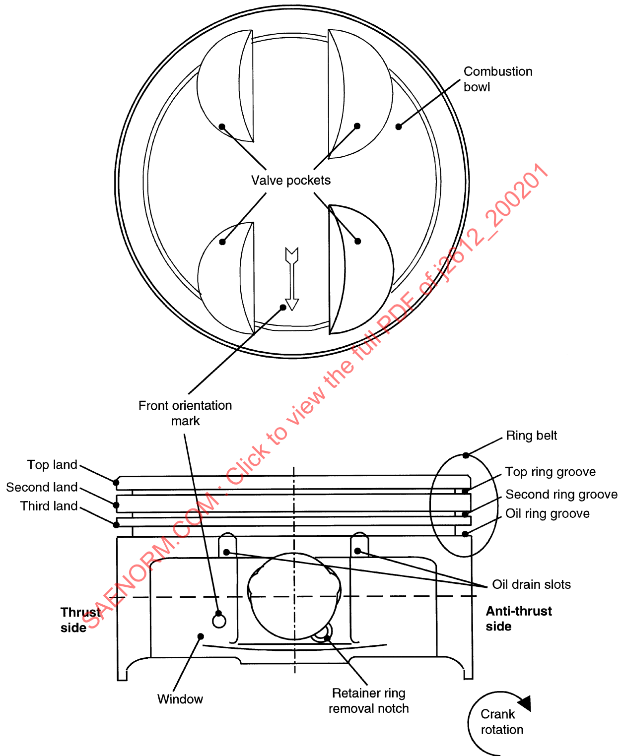
FIGURE 11—LIGHT DUTY MONOBLOCK PISTON — TOP AND SIDE VIEW
