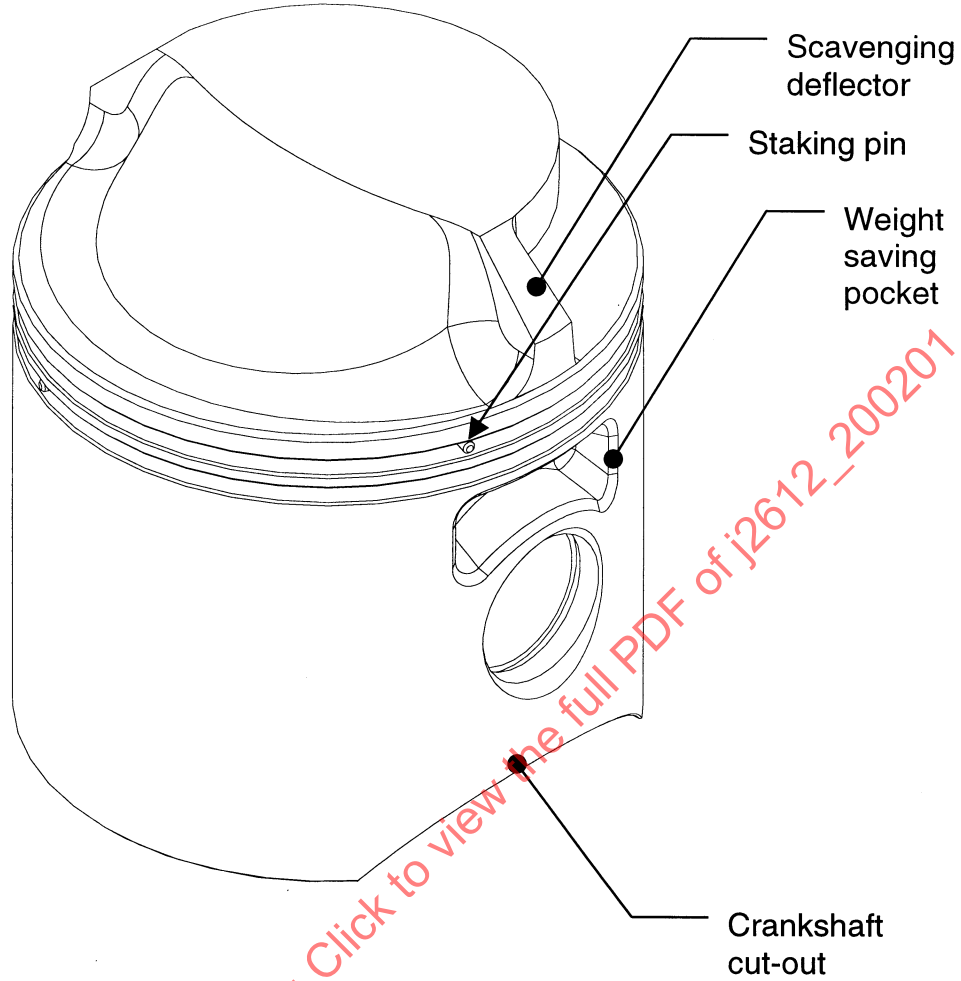
FIGURE 16—TWO-STROKE CROSS SCAVENGED PISTON
