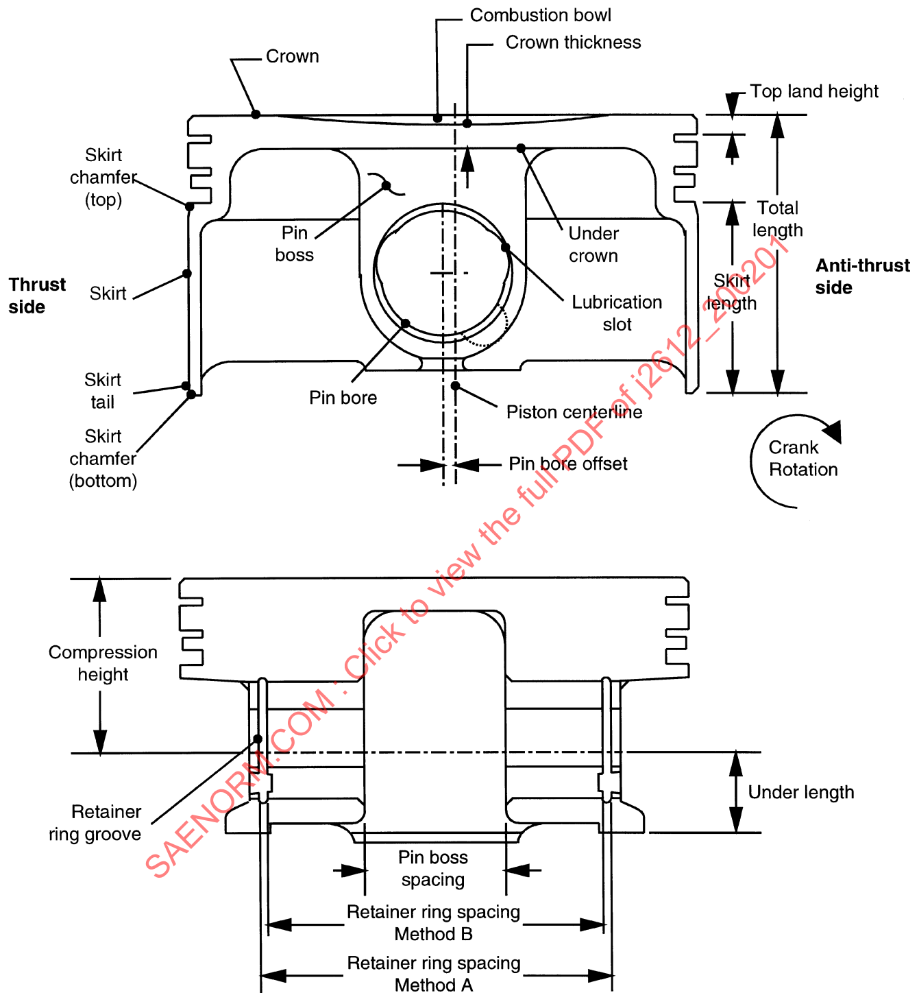
FIGURE 12—LIGHT DUTY MONOBLOCK PISTON: CUTAWAY VIEWS
