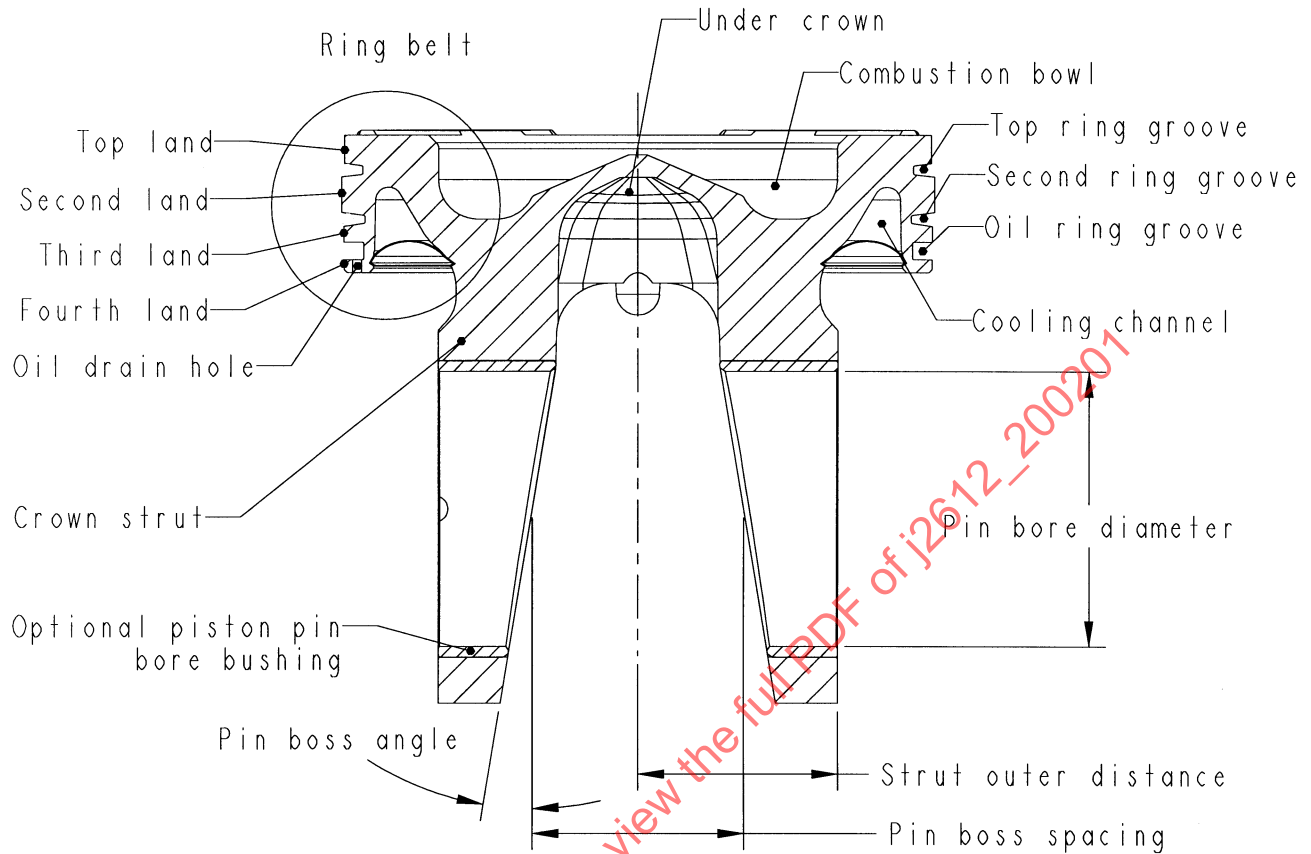
FIGURE 2—ARTICULATED PISTON CROWN – VIEW ALONG THRUST AXIS
