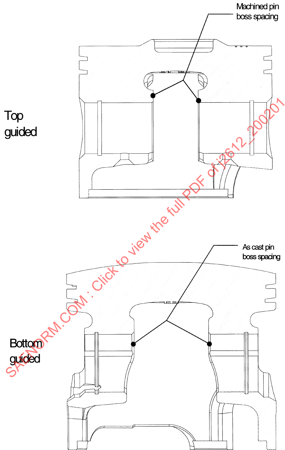
FIGURE 17—COMPARISONS OF PISTON DESIGN FOR TOP GUIDED/BOTTOM GUIDED CONNECTING RODS
