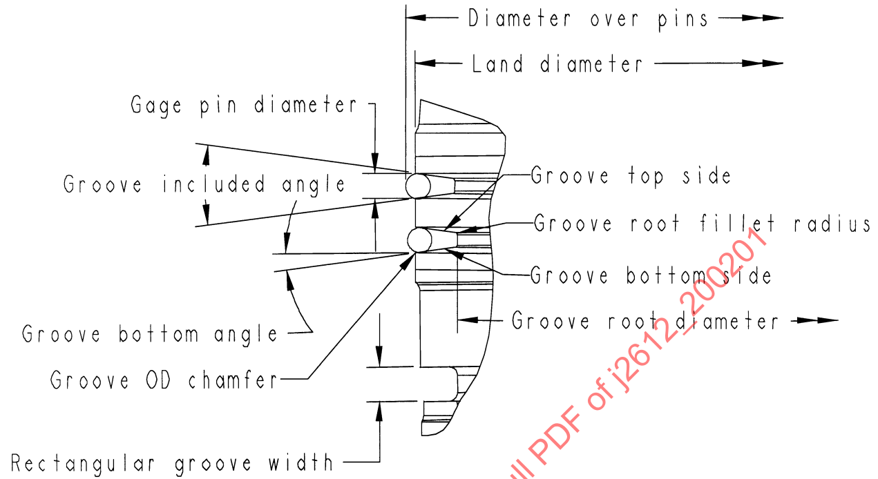
FIGURE 9—MEDIUM/HEAVY DUTY MONOBLOCK PISTON: RING BELT REGION
