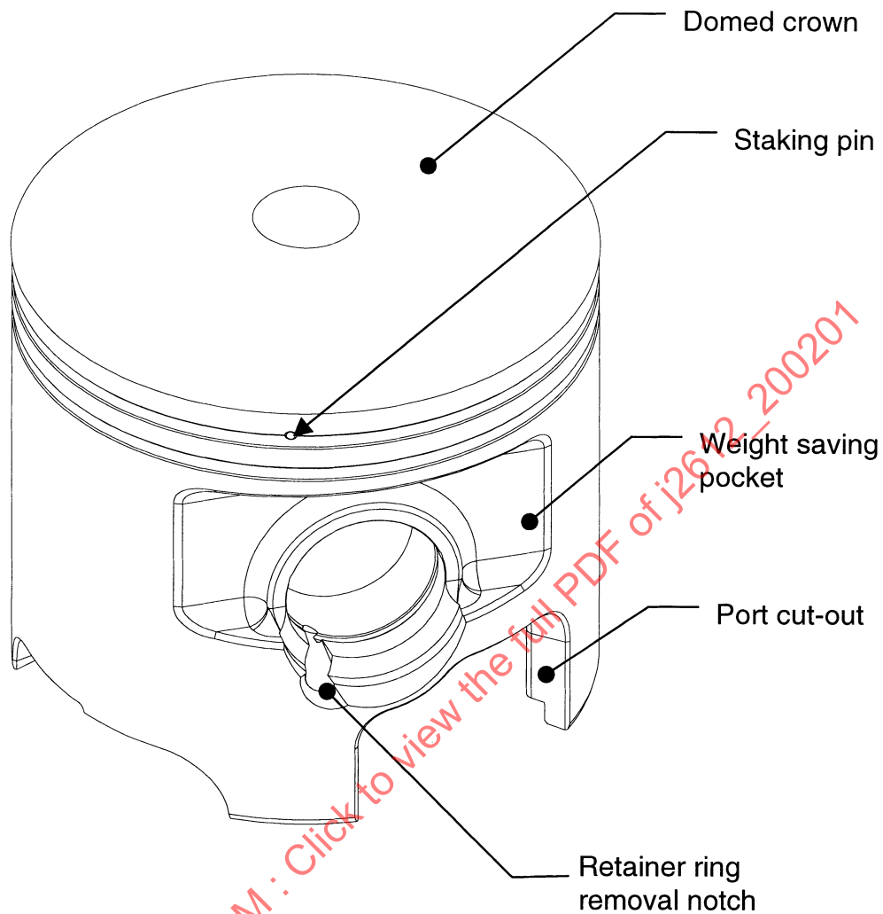
FIGURE 15—TWO-STROKE ELECTRONIC FUEL INJECTION PISTON (LOOP SCAVENGED)
