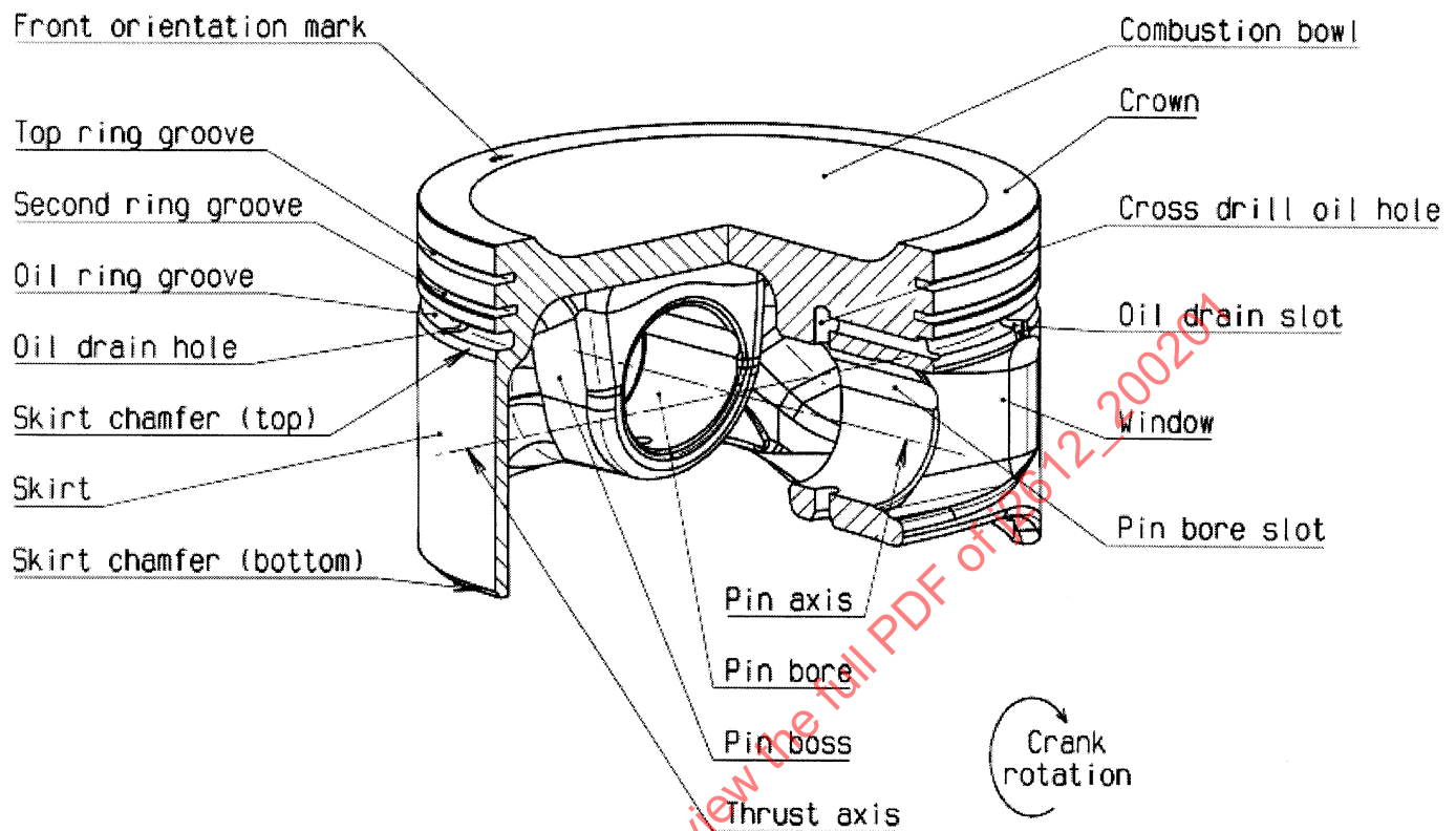
FIGURE 10—LIGHT DUTY MONOBLOCK PISTON — ISOMETRIC VIEW
