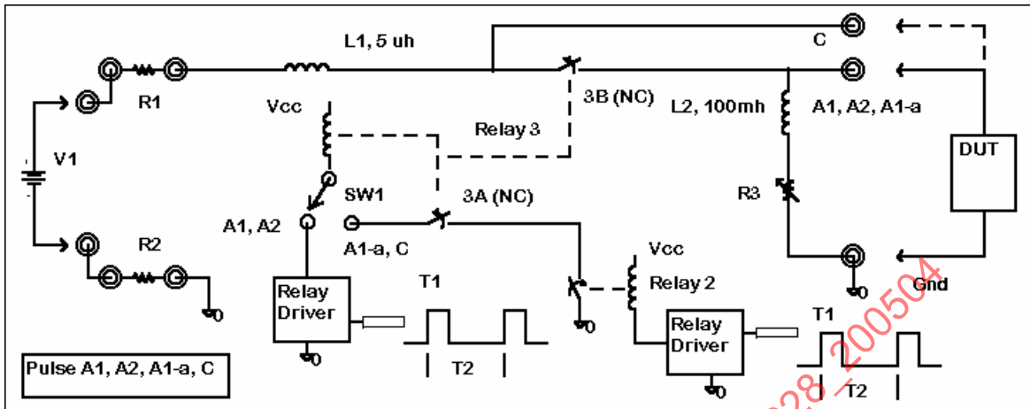
FIGURE 3—PULSE A1, A2, A1-A, C SCHEMATIC
