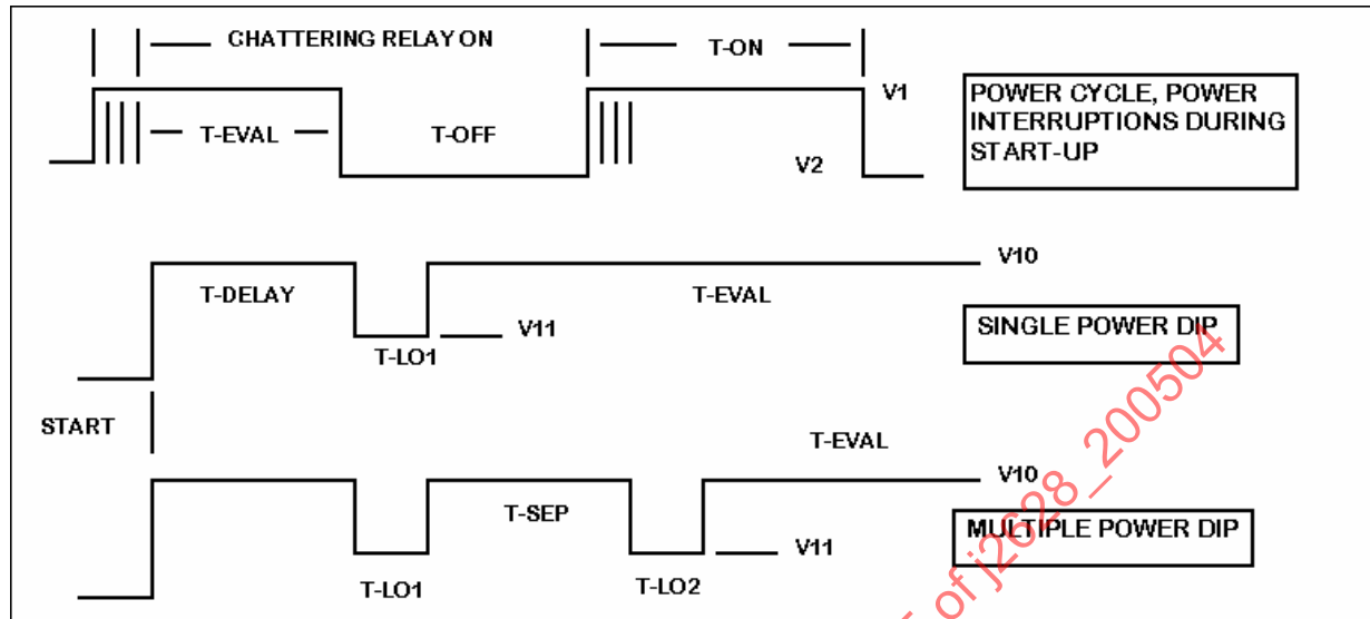
FIGURE 12—TIMING DIAGRAM
