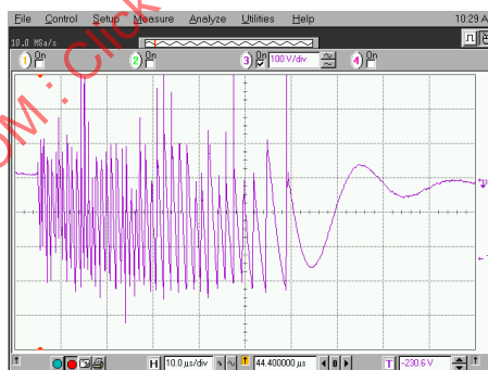
FIGURE 8—EXAMPLE OF A2 (10us, 100v), MINIMAL TRANSIENT WHEN LOADED
