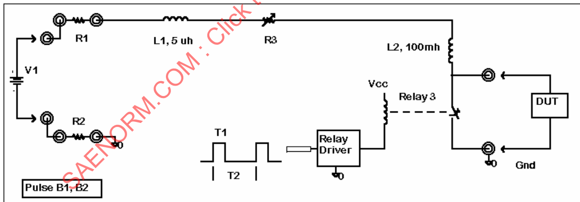
FIGURE 4—PULSE B1,B2 SCHEMATIC
