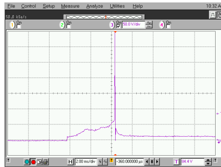
FIGURE 9A—EXAMPLE OF B1 (2ms, 50v)
