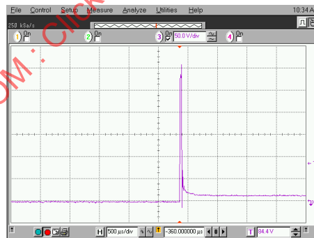
FIGURE 10—EXAMPLE OF B2 (500us, 50v) MINIMAL TRANSIENT WHEN LOADED
