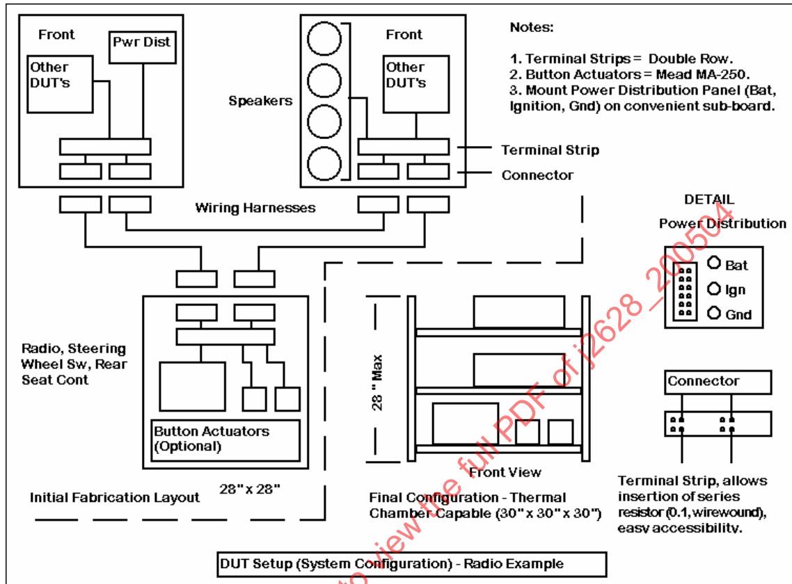
FIGURE 14—DUT SETUP - SYSTEM CONFIGURATION
