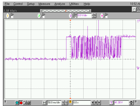
FIGURE 5—EXAMPLE OF POWER INTERRUPTIONS AT START UP (50ms, 5v)
