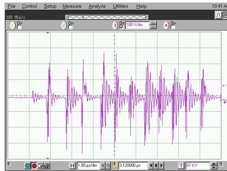
FIGURE 11A—EXAMPLE OF C (1 \mu s, 100v)
