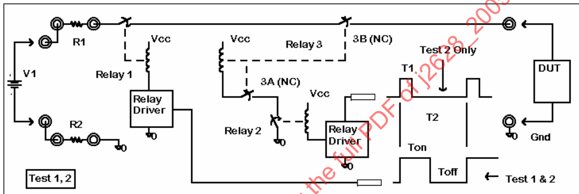
FIGURE 2—TEST 1,2 SCHEMATIC
