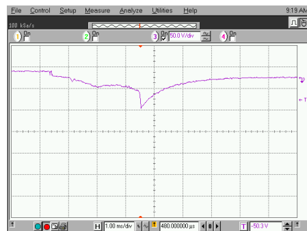
FIGURE 6B—A1 LOADED (1ms, 50v)
