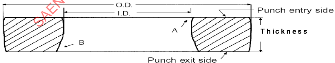
FIGURE 2—Washer Profile (Exaggerated for Clarity)
