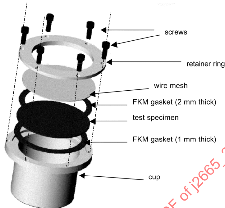
FIGURE 2 - EXPLODED VIEW OF THE MODIFIED THWING-ALBERT PERMEATION CUP, SHOWING THE ASSEMBLY SEQUENCE OF THE COMPONENTS
