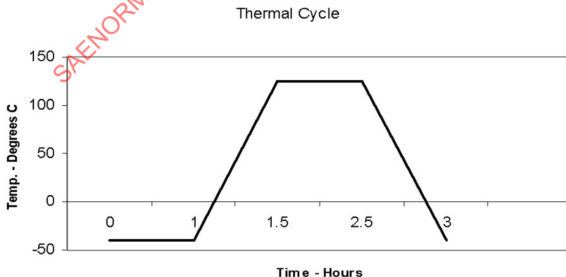
Figure 6 - Thermal cycling temperature profile
