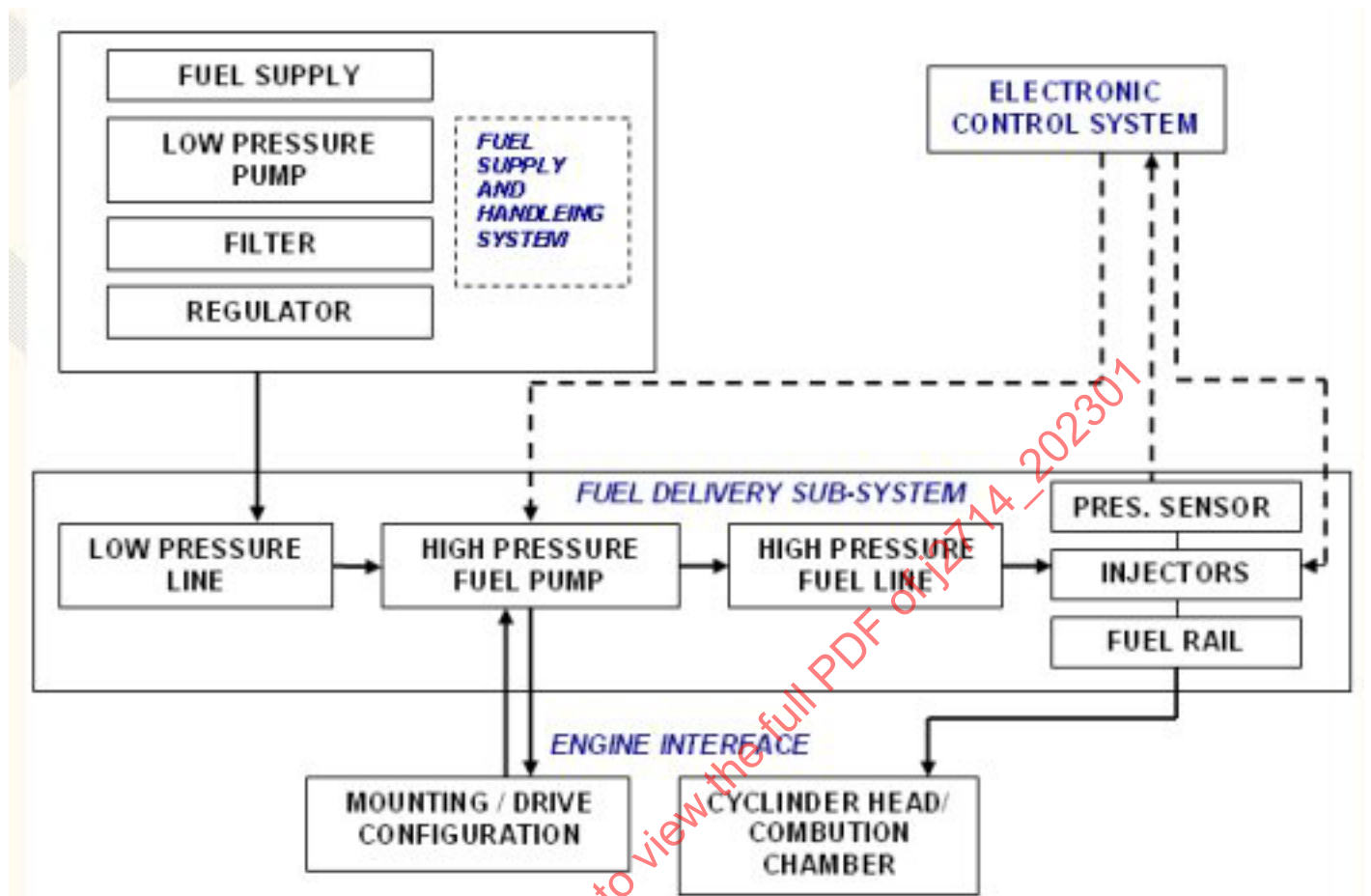
Figure A1 - Direction injection gasoline high-pressure pump, system interface block diagram
