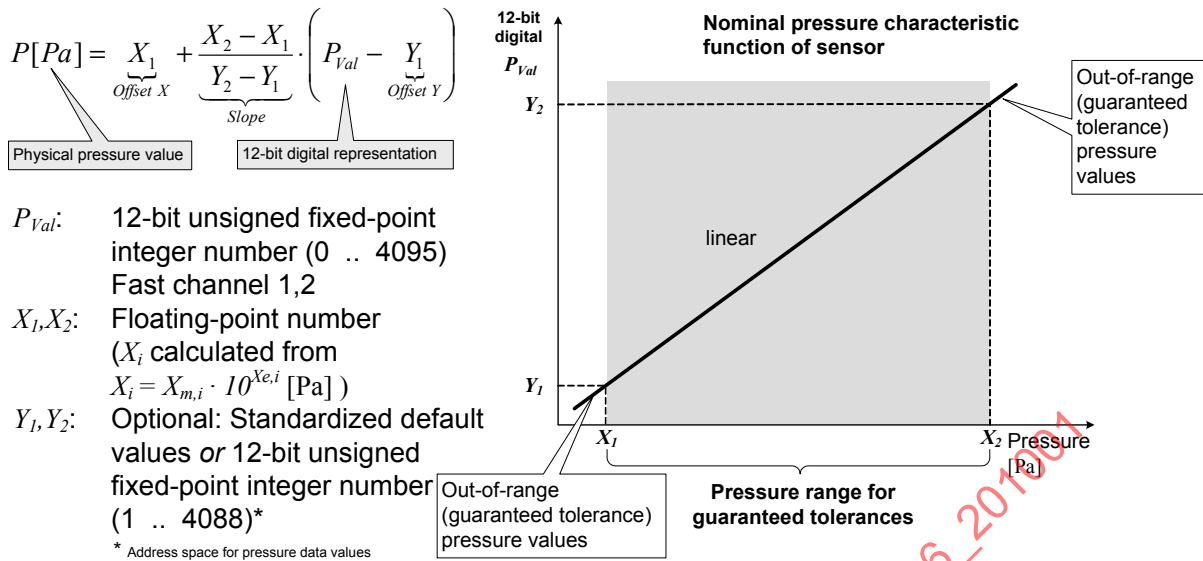
FIGURE A.5.3.1.1-1 - PRESSURE TRANSFER CHARACTERISTIC CURVE
