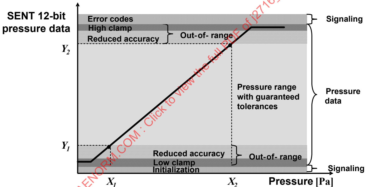
FIGURE A.5.3.1.3-1 - GUARANTEED PRESSURE RANGE, OUT-OF-RANGE VALUES AND SIGNALING DATA
