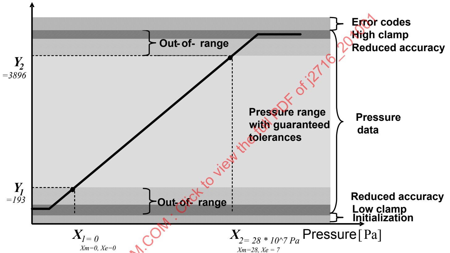
FIGURE A.5.5.1-1 - APPLICATION WITH DEFAULT Y_1, Y_2
