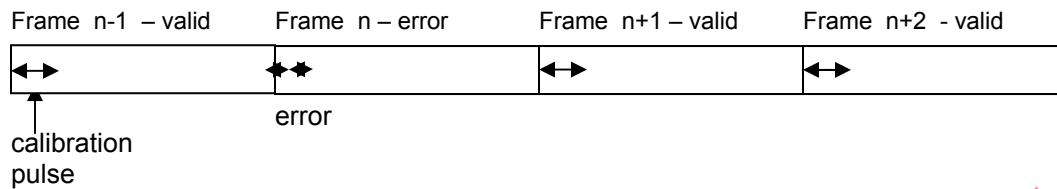
FIGURE 5.3.3.1-1 - ERROR PATTERN FOR SUCCESSIVE CALIBRATION PULSE DETECTION.
