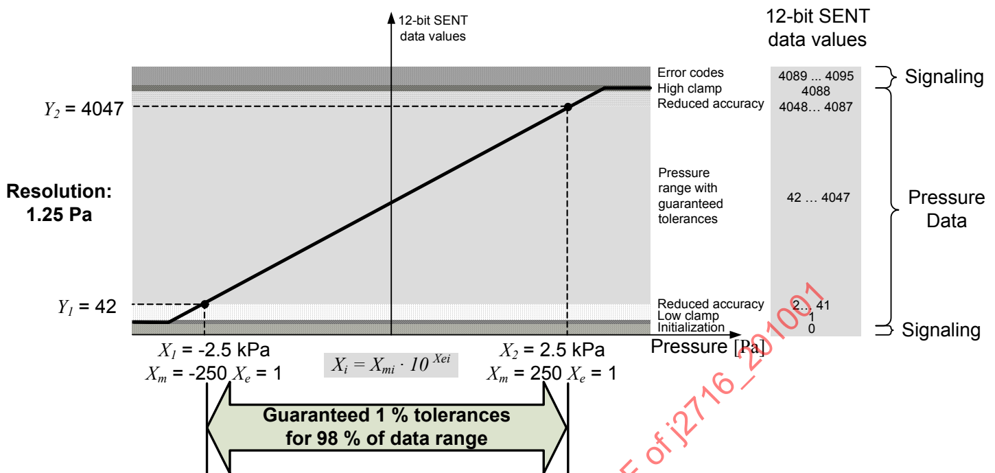
FIGURE A.5.5.2-1 - APPLICATION WITH SENSOR-SPECIFIC Y_1 , Y_2
