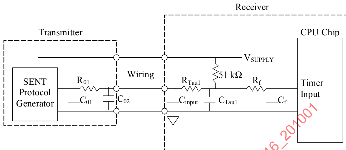
FIGURE 6.3-3 – EXAMPLE LEGACY SENT SYSTEM INTERFACE CIRCUIT TOPOLOGY
