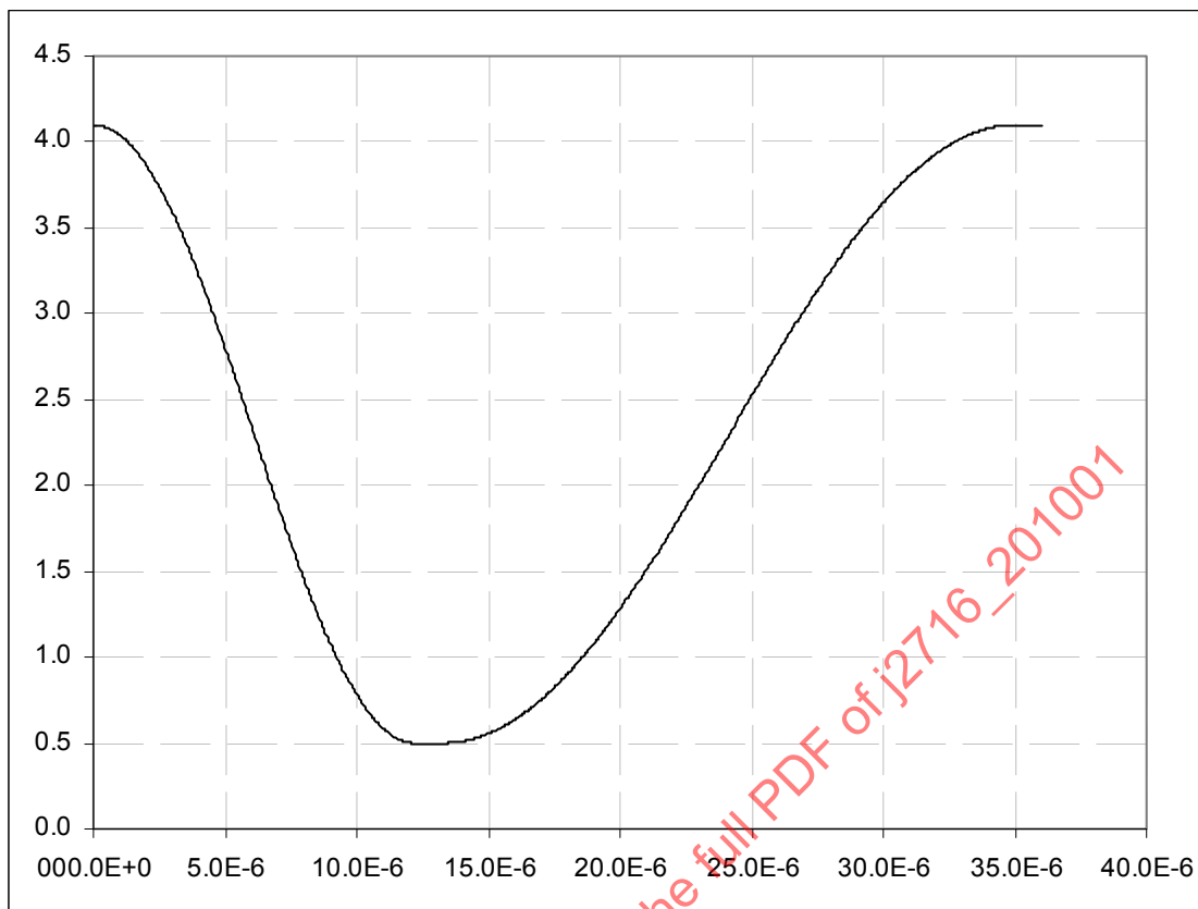
FIGURE 6.3.1-1 – EXAMPLE SENT SHAPED WAVEFORM TRANSMITTER OUTPUT
