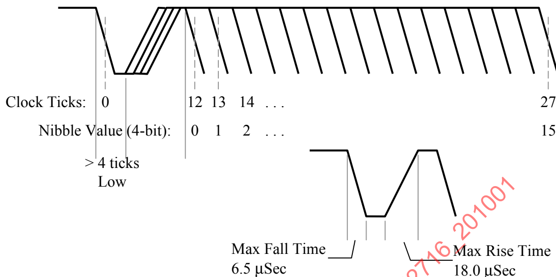
FIGURE 5.2.3-1 – EXAMPLE NOMINAL NIBBLE TIMES
