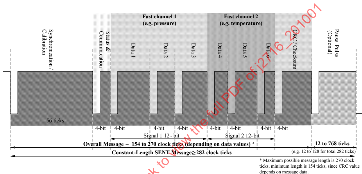
FIGURE A.5.1-1 - DATA CHANNELS FOR PRESSURE SENSORS AND COMBINED PRESSURE AND TEMPERATURE SENSORS
