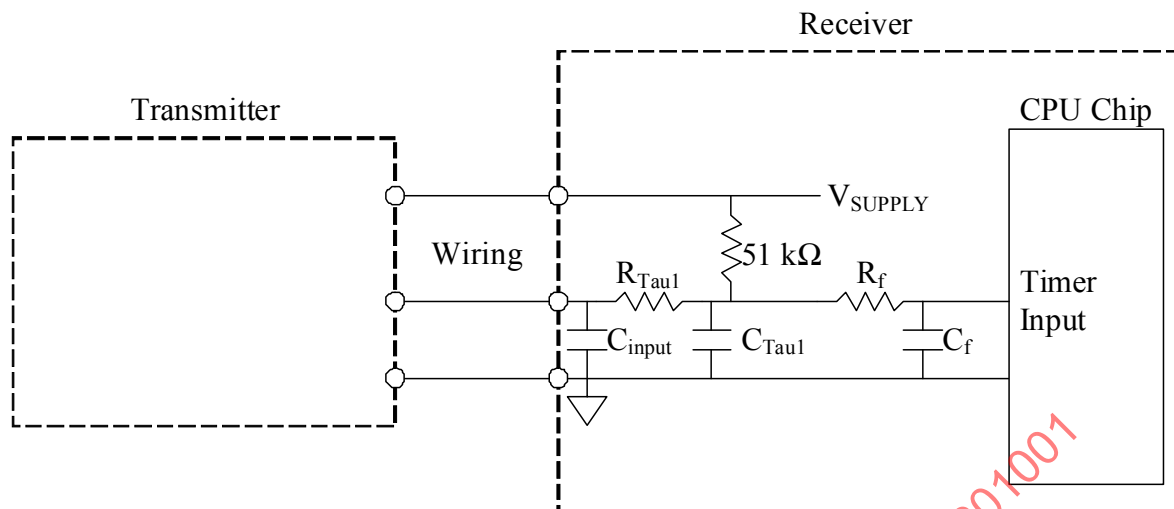
FIGURE 6.3-1 – LEGACY SENT RECEIVER INTERFACE CIRCUIT TOPOLOGY
