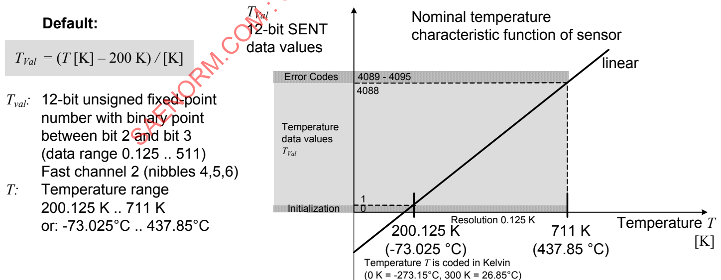
FIGURE A.5.3.2-1 - DEFAULT TEMPERATURE CHARACTERISTIC FUNCTION
