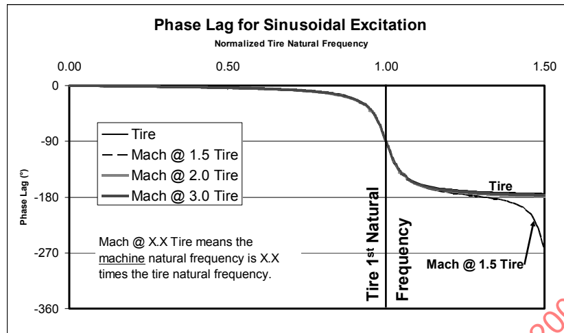
FIGURE 5 - ILLUSTRATION OF THE PHASE EFFECT OF A MACHINE RESONANCE
