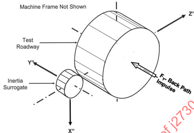
FIGURE 11 - INPUTTING AN F_{Y''} IMPULSE INTO THE BACK PATH WITH A MODAL HAMMER
