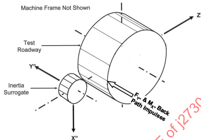
FIGURE 15 - INPUTTING BOTH F_{Y''} AND M_{X''} IMPULSES INTO THE BACK PATH WITH A MODAL HAMMER
