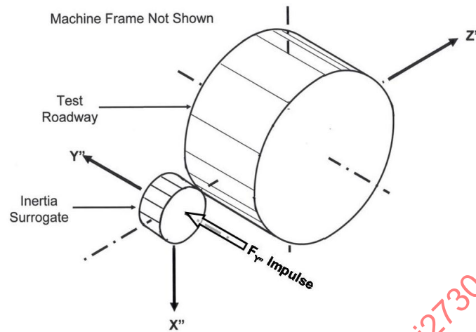
FIGURE 6 - INPUTTING AN F_{Y''} IMPULSE WITH A MODAL HAMMER
