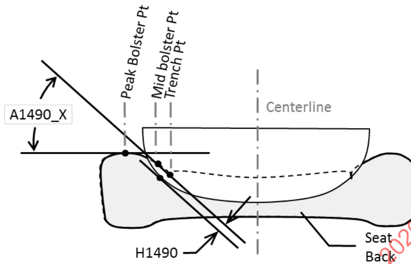
Figure 7F - Seat back lateral cross-section dimensions
