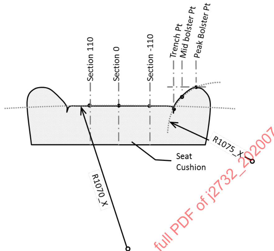
Figure 5B - Seat cushion lateral cross-section dimensions
