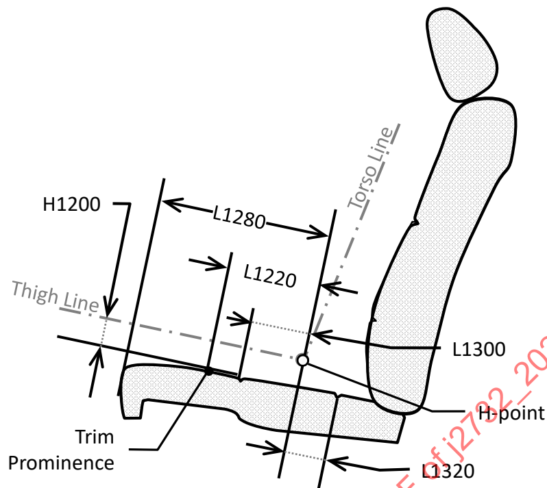
Figure 6A - Seat cushion centerline section
