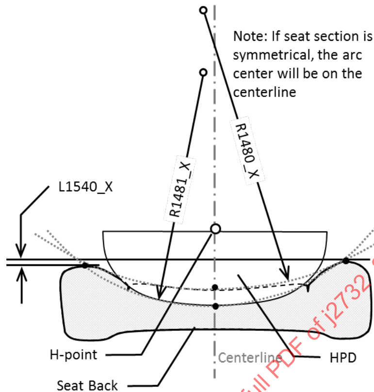
Figure 7D - Seat back lateral cross-section - bolster asymmetry and radial dimensions
