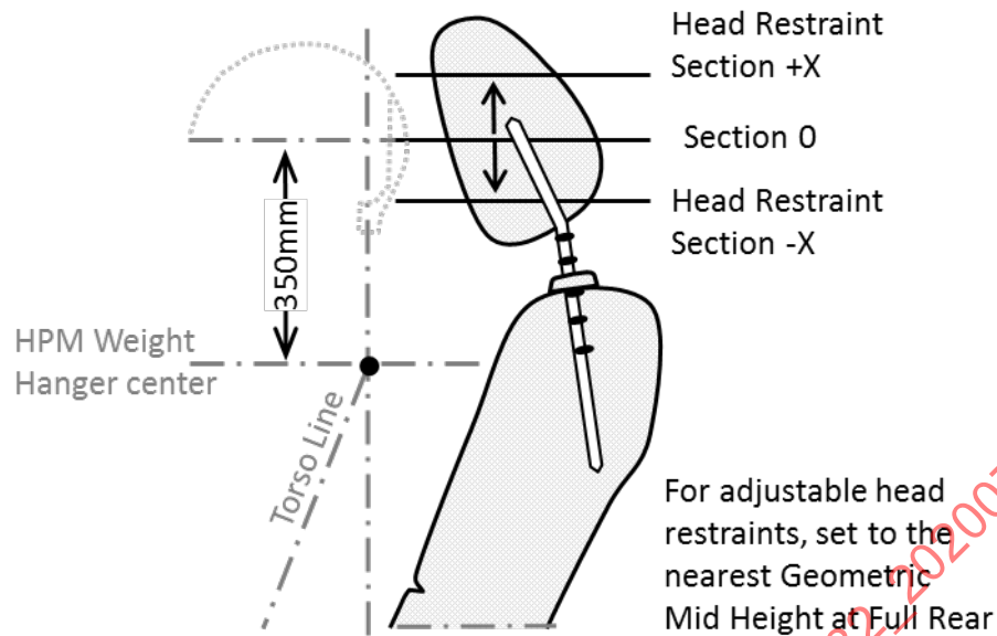
Figure 4B - Cross sections head restraint sections
