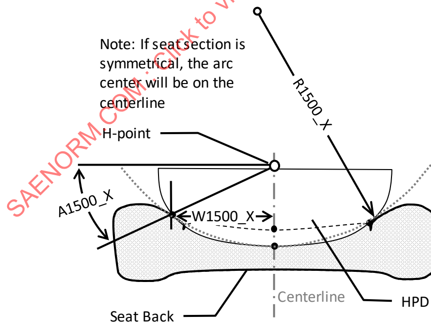
Figure 7D - Seat back lateral cross-section - bolster asymmetry and radial dimensions
