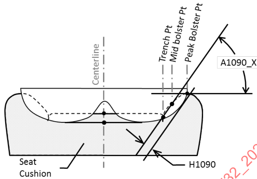
Figure 5F - Seat cushion lateral cross-section dimensions
