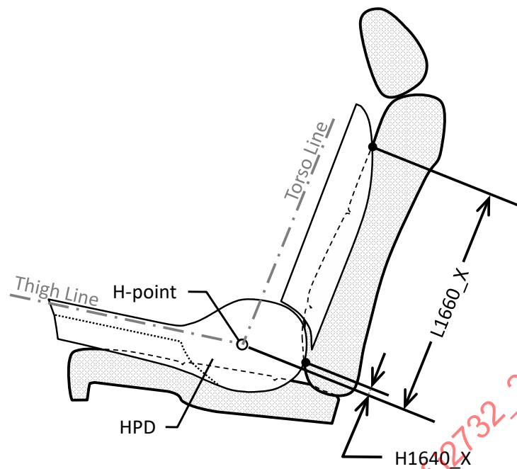
Figure 8B - HPD-specific seat back centerline section dimensions
