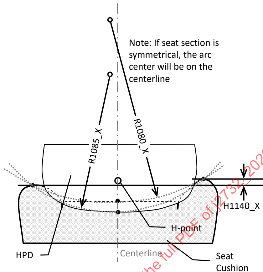
Figure 5D - Seat cushion lateral cross-section - bolster asymmetry and radial dimensions
