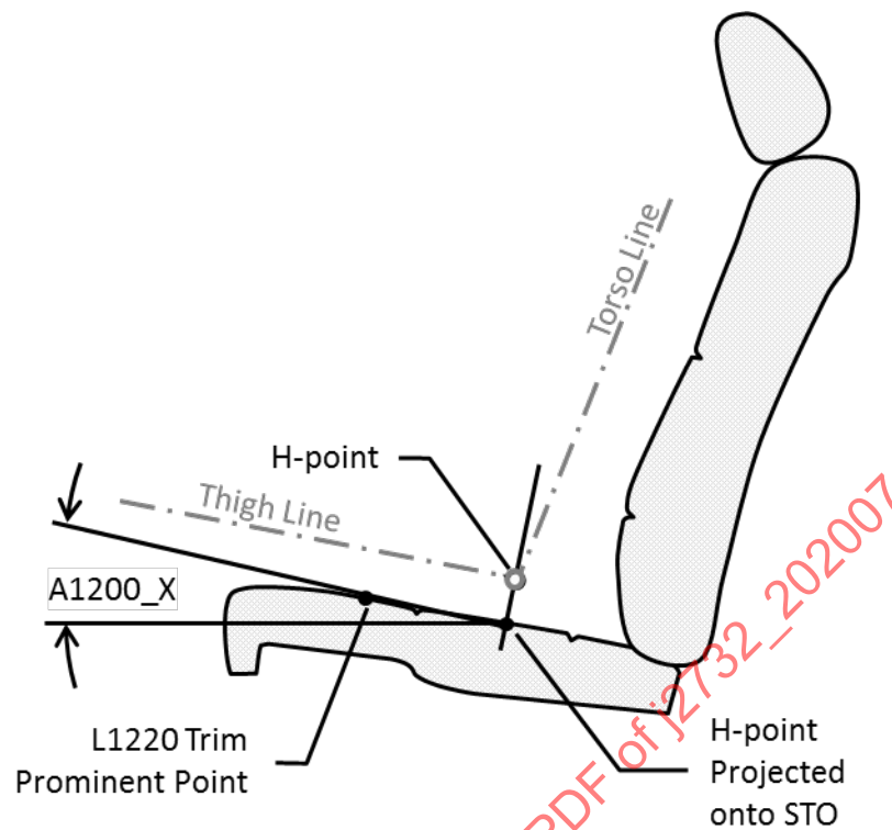
Figure 6C - Seat cushion centerline section
