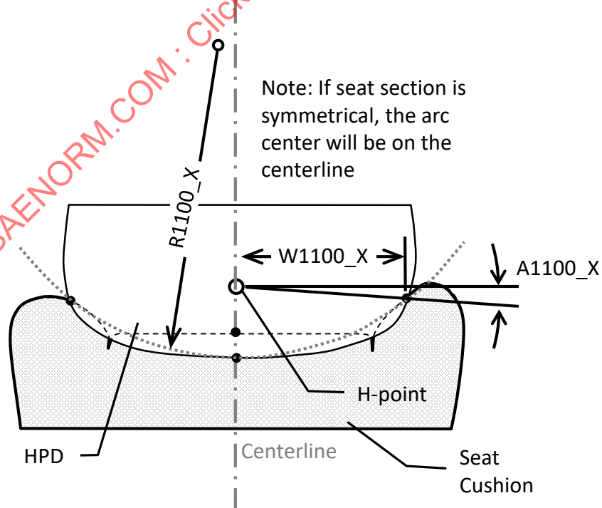
Figure 5E - Seat cushion lateral cross-section dimensions
