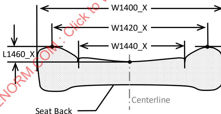
Figure 7A - Seat back lateral cross-section dimensions
