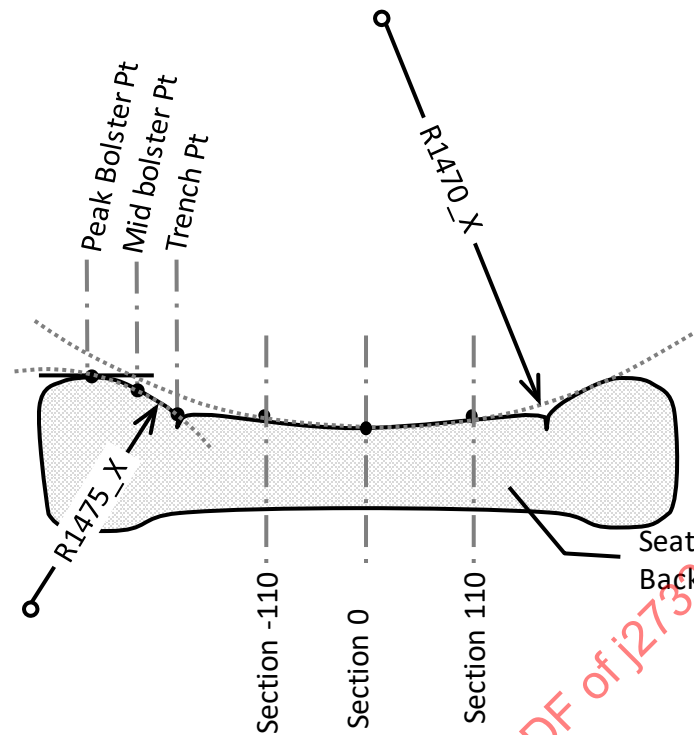
Figure 7B - Seat back lateral cross-section dimensions
