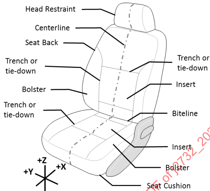
Figure 1 - General seat definitions
