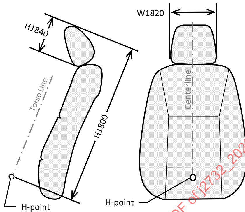
Figure 9A - Head restraint dimensions
